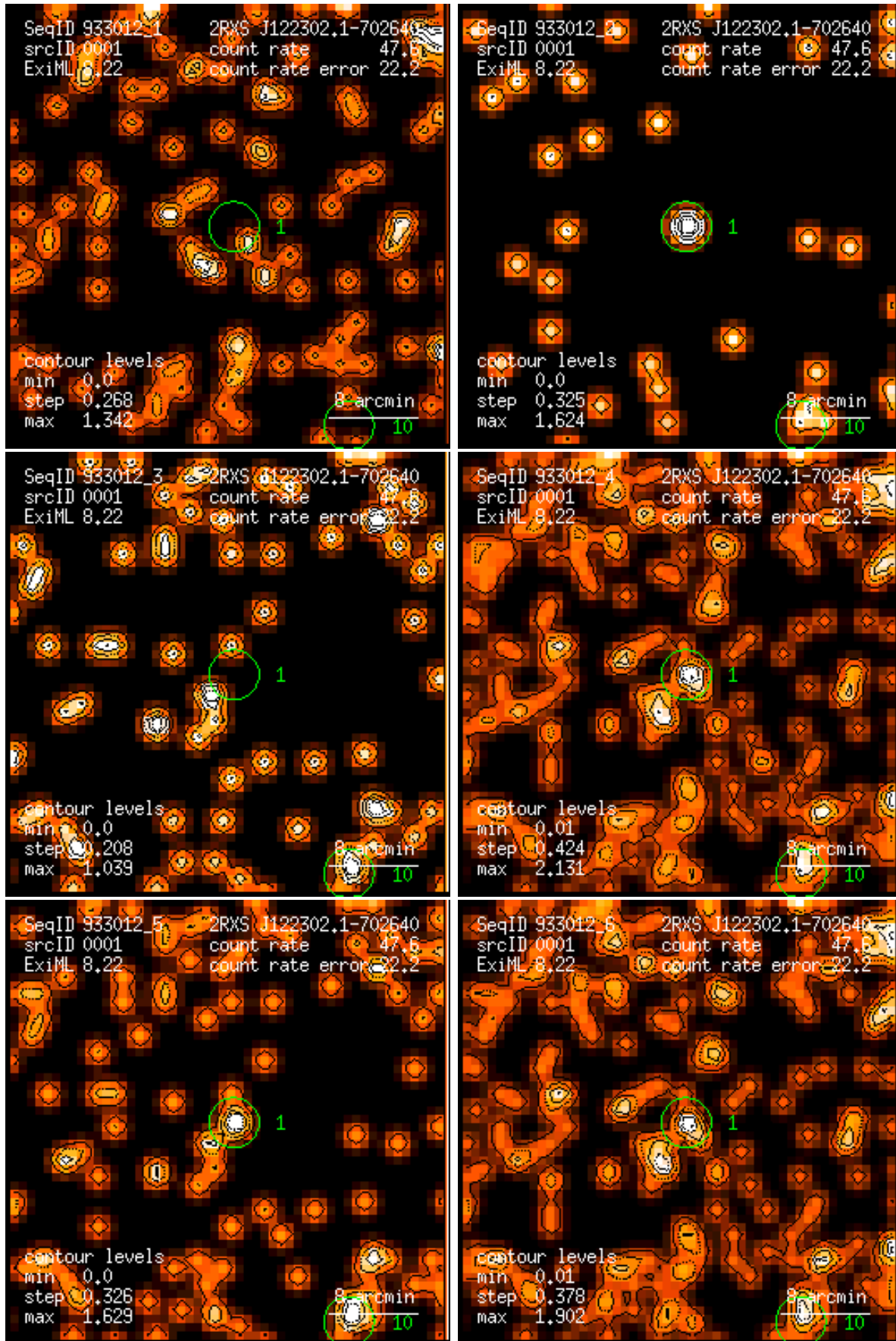
Figure 1: RASS 933012: detection 0001: band rate images, Gaussian filter: (1) PSPC channels 11 – 41, (2) 52 – 90, (3) 91 – 201, (4) 11 – 235, (5) 52 – 201, (6) 11 – 201. Broad band rates in counts/ks. Band rate contour levels in counts/ks/arcmin 2 .
