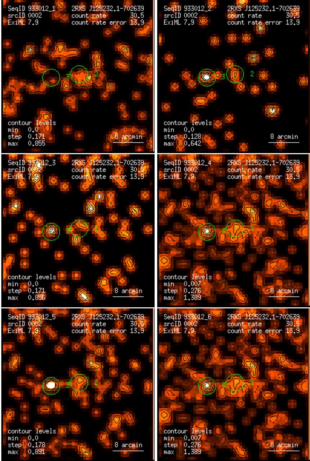
Figure 2: RASS 933012: detection 0002: band rate images, Gaussian filter: (1) PSPC channels 11 – 41, (2) 52 – 90, (3) 91 – 201, (4) 11 – 235, (5) 52 – 201, (6) 11 – 201. Broad band rates in counts/ks. Band rate contour levels in counts/ks/arcmin 2 .
