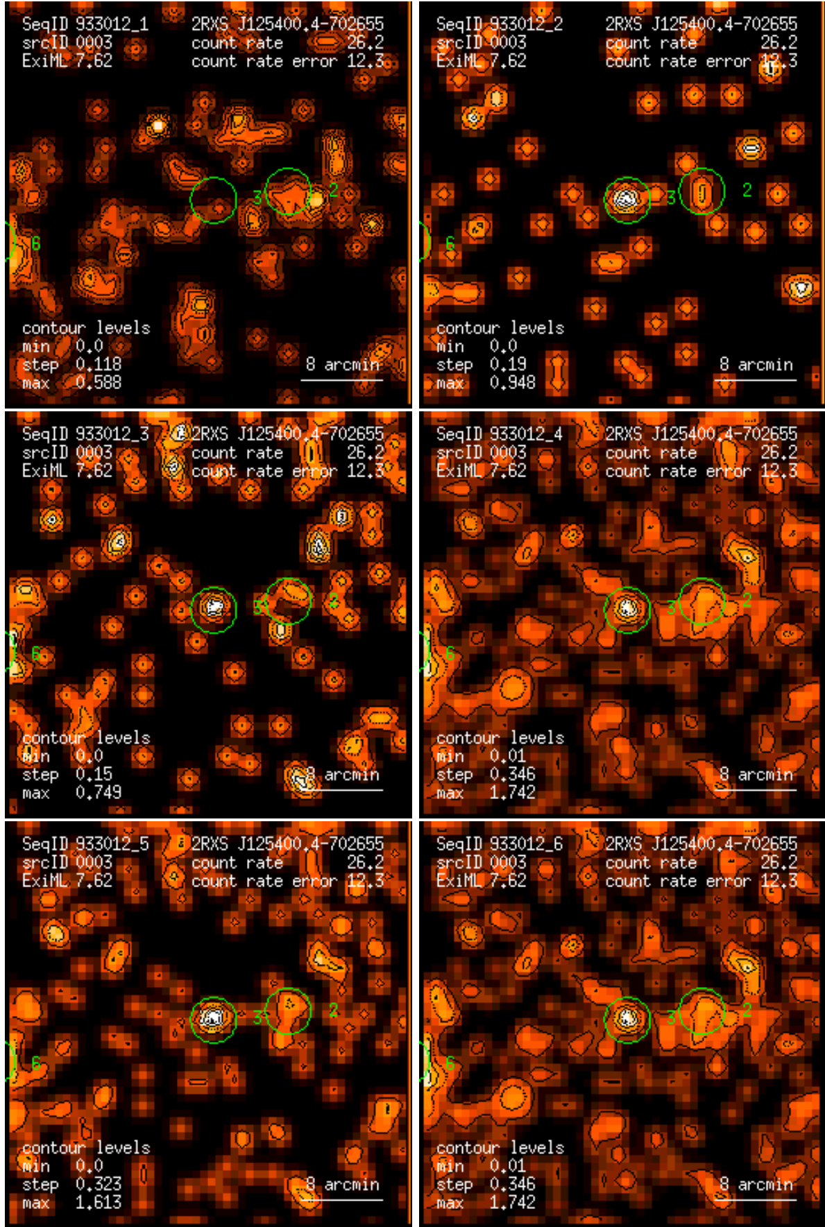
Figure 3: RASS 933012: detection 0003: band rate images, Gaussian filter: (1) PSPC channels 11 – 41, (2) 52 – 90, (3) 91 – 201, (4) 11 – 235, (5) 52 – 201, (6) 11 – 201. Broad band rates in counts/ks. Band rate contour levels in counts/ks/arcmin 2 .
