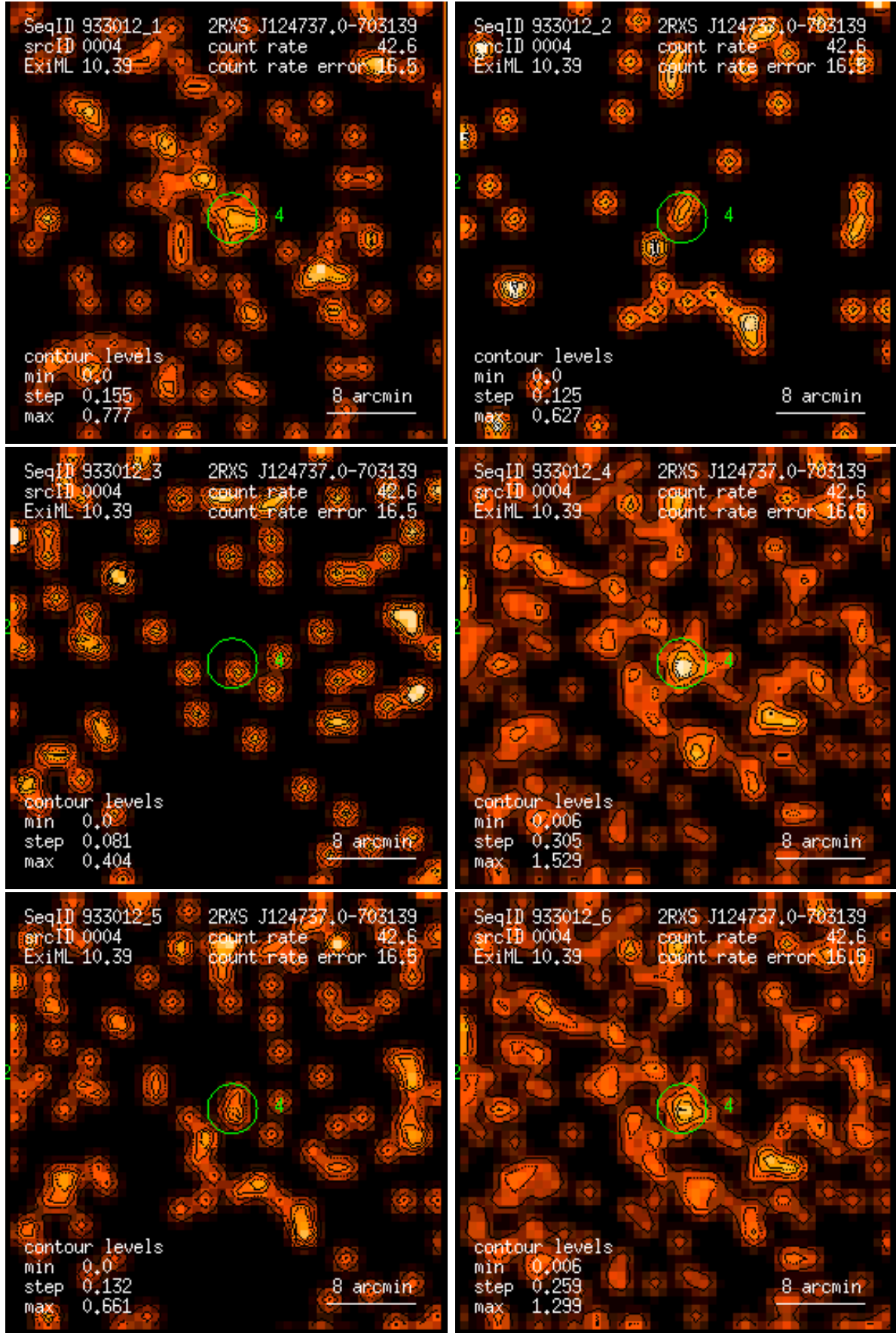
Figure 4: RASS 933012: detection 0004: band rate images, Gaussian filter: (1) PSPC channels 11 – 41, (2) 52 – 90, (3) 91 – 201, (4) 11 – 235, (5) 52 – 201, (6) 11 – 201. Broad band rates in counts/ks. Band rate contour levels in counts/ks/arcmin 2 .
