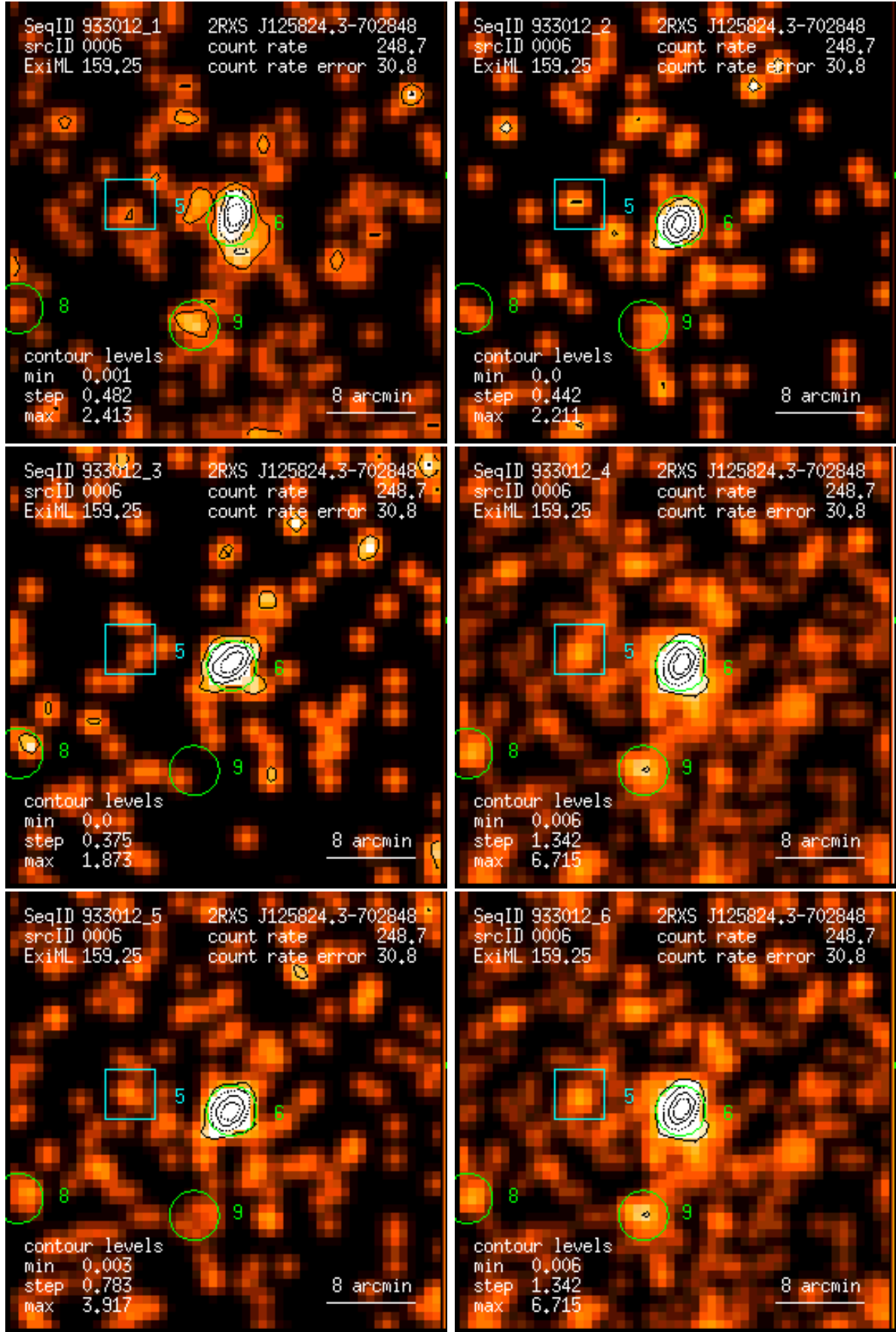
Figure 6: RASS 933012: detection 0006: band rate images, Gaussian filter: (1) PSPC channels 11 – 41, (2) 52 – 90, (3) 91 – 201, (4) 11 – 235, (5) 52 – 201, (6) 11 – 201. Broad band rates in counts/ks. Band rate contour levels in counts/ks/arcmin 2 .
