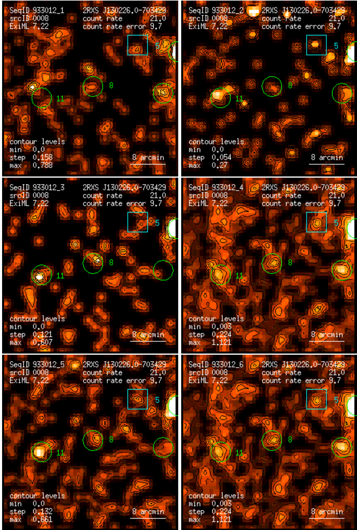
Figure 8: RASS 933012: detection 0008: band rate images, Gaussian filter: (1) PSPC channels 11 – 41, (2) 52 – 90, (3) 91 – 201, (4) 11 – 235, (5) 52 – 201, (6) 11 – 201. Broad band rates in counts/ks. Band rate contour levels in counts/ks/arcmin 2 .
