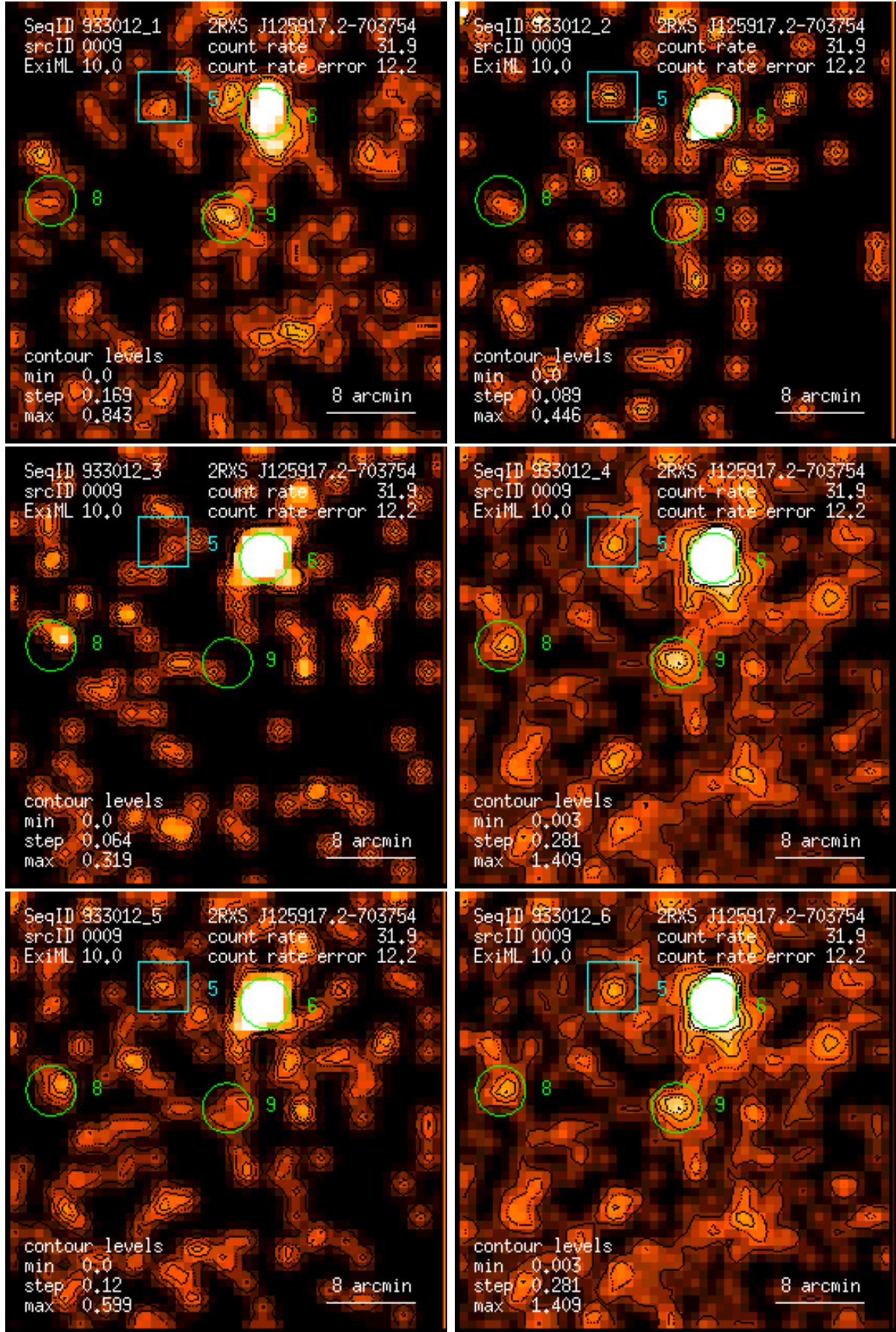
Figure 9: RASS 933012: detection 0009: band rate images, Gaussian filter: (1) PSPC channels 11 – 41, (2) 52 – 90, (3) 91 – 201, (4) 11 – 235, (5) 52 – 201, (6) 11 – 201. Broad band rates in counts/ks. Band rate contour levels in counts/ks/arcmin 2 .
