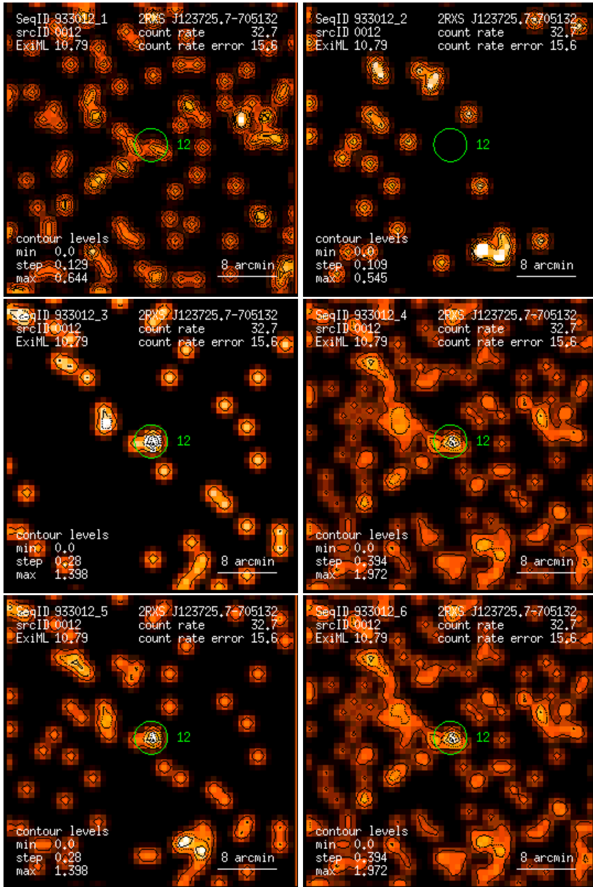
Figure 12: RASS 933012: detection 0012: band rate images, Gaussian filter: (1) PSPC channels 11 – 41, (2) 52 – 90, (3) 91 – 201, (4) 11 – 235, (5) 52 – 201, (6) 11 – 201. Broad band rates in counts/ks. Band rate contour levels in counts/ks/arcmin 2 .
