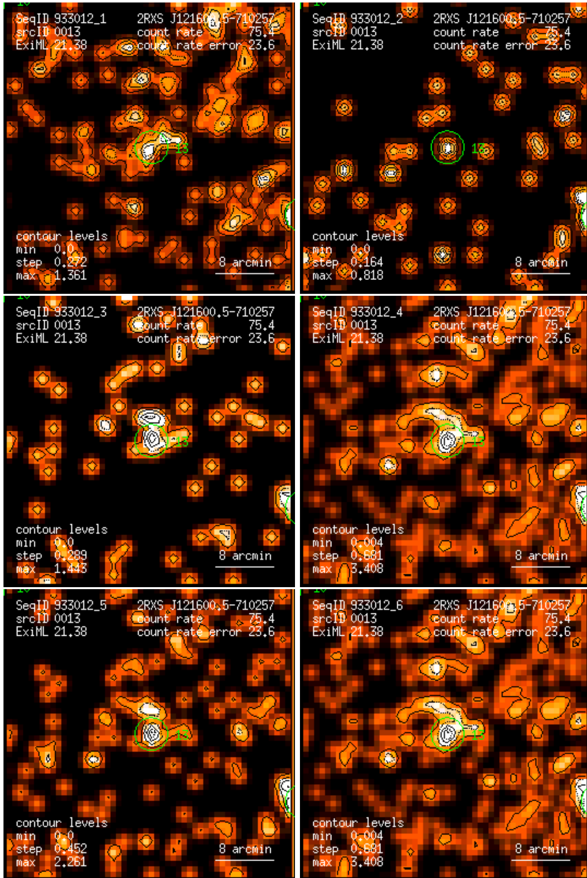
Figure 13: RASS 933012: detection 0013: band rate images, Gaussian filter: (1) PSPC channels 11 – 41, (2) 52 – 90, (3) 91 – 201, (4) 11 – 235, (5) 52 – 201, (6) 11 – 201. Broad band rates in counts/ks. Band rate contour levels in counts/ks/arcmin 2 .
