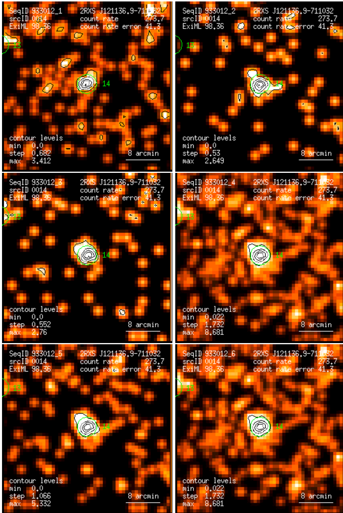
Figure 14: RASS 933012: detection 0014: band rate images, Gaussian filter: (1) PSPC channels 11 – 41, (2) 52 – 90, (3) 91 – 201, (4) 11 – 235, (5) 52 – 201, (6) 11 – 201. Broad band rates in counts/ks. Band rate contour levels in counts/ks/arcmin 2 .
