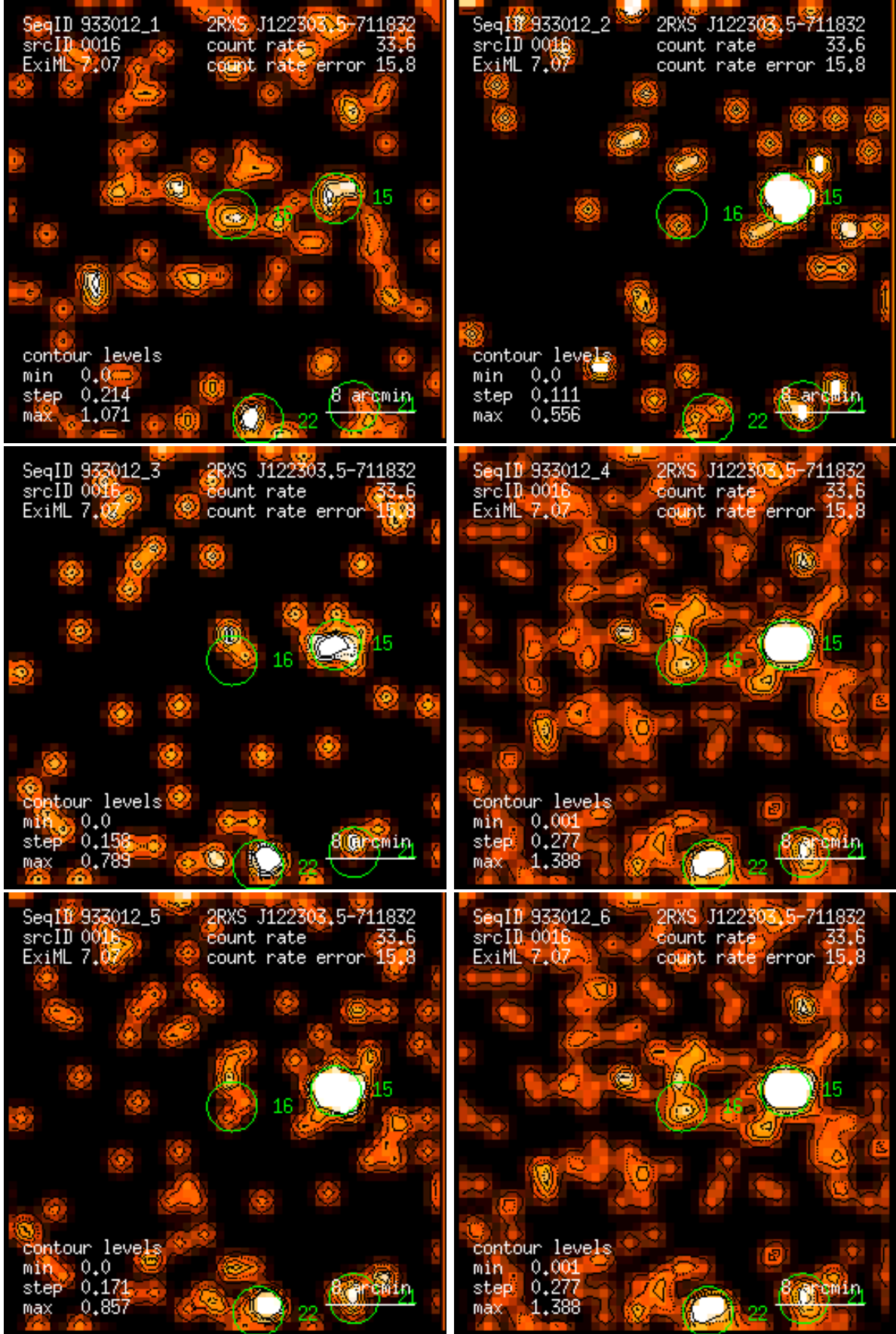
Figure 16: RASS 933012: detection 0016: band rate images, Gaussian filter: (1) PSPC channels 11 – 41, (2) 52 – 90, (3) 91 – 201, (4) 11 – 235, (5) 52 – 201, (6) 11 – 201. Broad band rates in counts/ks. Band rate contour levels in counts/ks/arcmin 2 .
