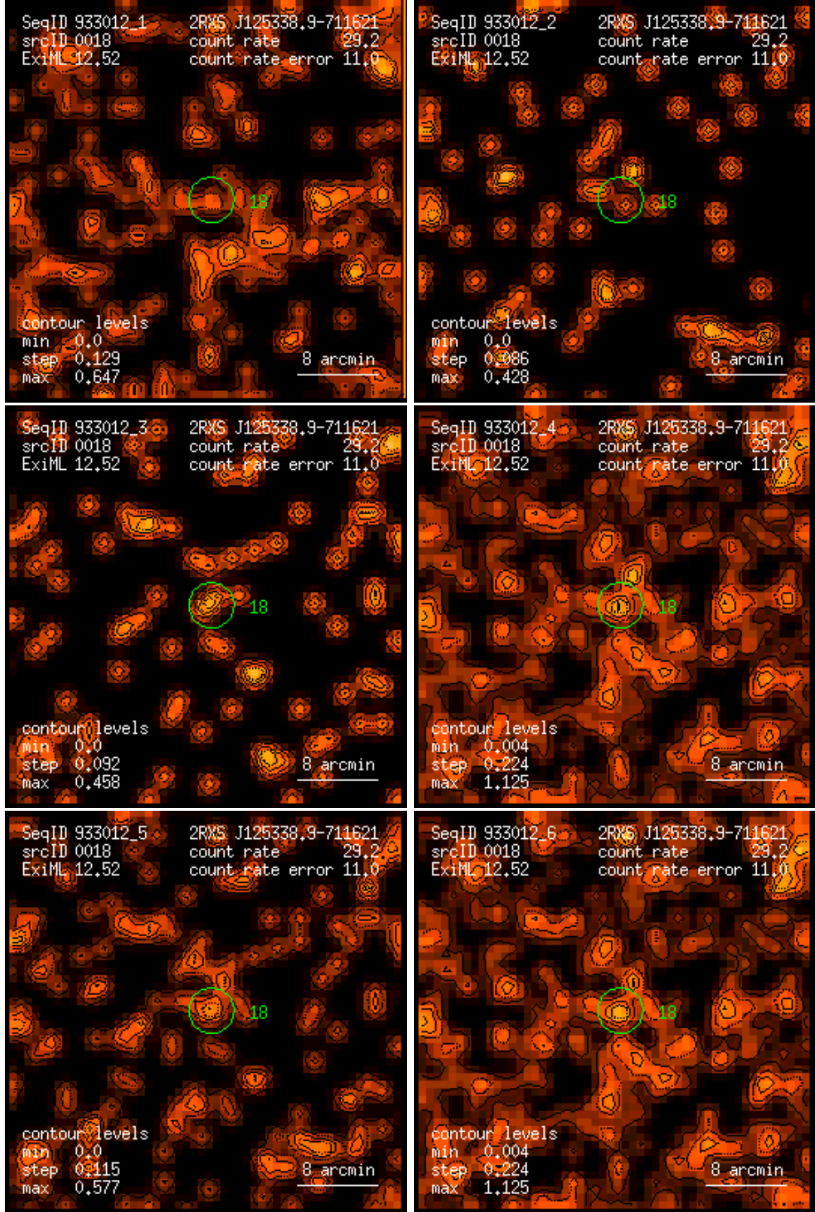
Figure 18: RASS 933012: detection 0018: band rate images, Gaussian filter: (1) PSPC channels 11 – 41, (2) 52 – 90, (3) 91 – 201, (4) 11 – 235, (5) 52 – 201, (6) 11 – 201. Broad band rates in counts/ks. Band rate contour levels in counts/ks/arcmin 2 .
