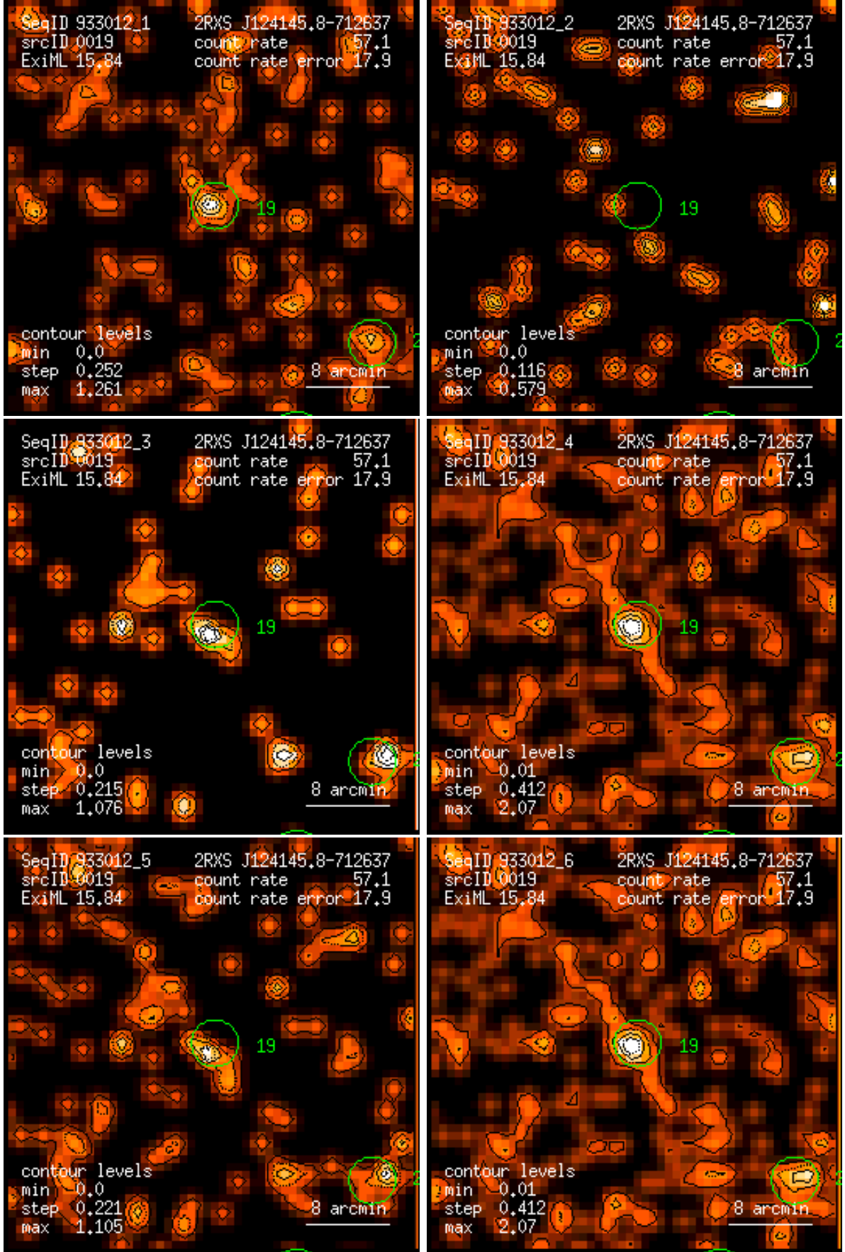
Figure 19: RASS 933012: detection 0019: band rate images, Gaussian filter: (1) PSPC channels 11 – 41, (2) 52 – 90, (3) 91 – 201, (4) 11 – 235, (5) 52 – 201, (6) 11 – 201. Broad band rates in counts/ks. Band rate contour levels in counts/ks/arcmin 2 .
