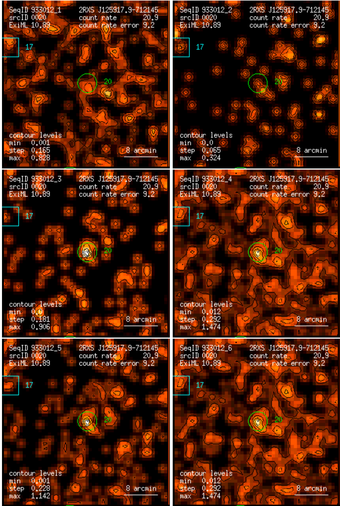
Figure 20: RASS 933012: detection 0020: band rate images, Gaussian filter: (1) PSPC channels 11 – 41, (2) 52 – 90, (3) 91 – 201, (4) 11 – 235, (5) 52 – 201, (6) 11 – 201. Broad band rates in counts/ks. Band rate contour levels in counts/ks/arcmin 2 .
