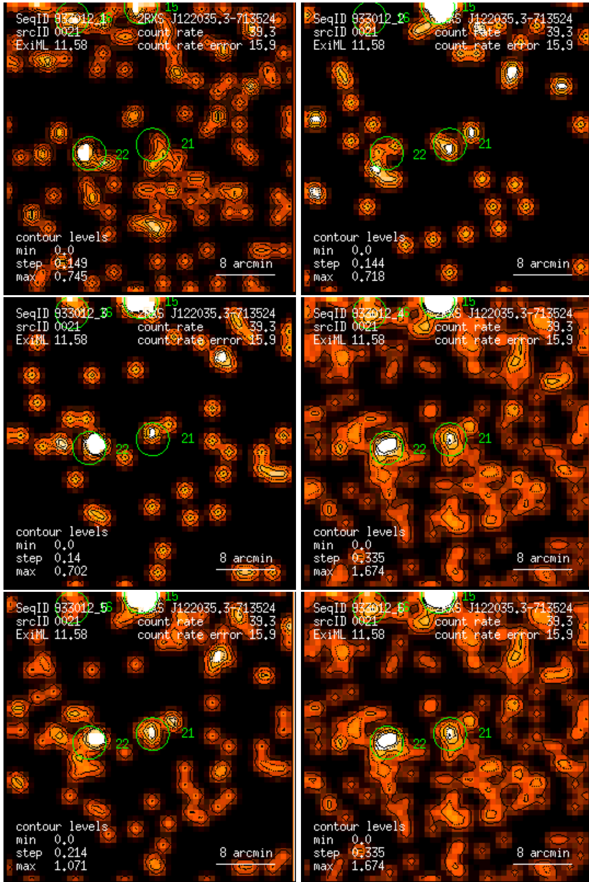
Figure 21: RASS 933012: detection 0021: band rate images, Gaussian filter: (1) PSPC channels 11 – 41, (2) 52 – 90, (3) 91 – 201, (4) 11 – 235, (5) 52 – 201, (6) 11 – 201. Broad band rates in counts/ks. Band rate contour levels in counts/ks/arcmin 2 .
