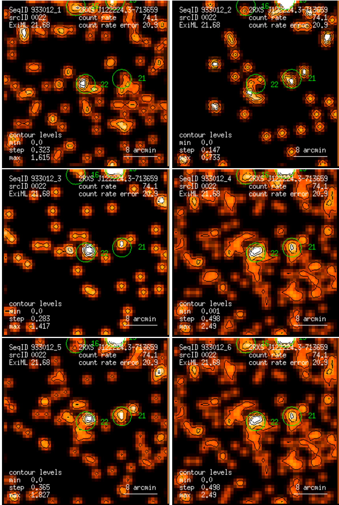
Figure 22: RASS 933012: detection 0022: band rate images, Gaussian filter: (1) PSPC channels 11 – 41, (2) 52 – 90, (3) 91 – 201, (4) 11 – 235, (5) 52 – 201, (6) 11 – 201. Broad band rates in counts/ks. Band rate contour levels in counts/ks/arcmin 2 .
