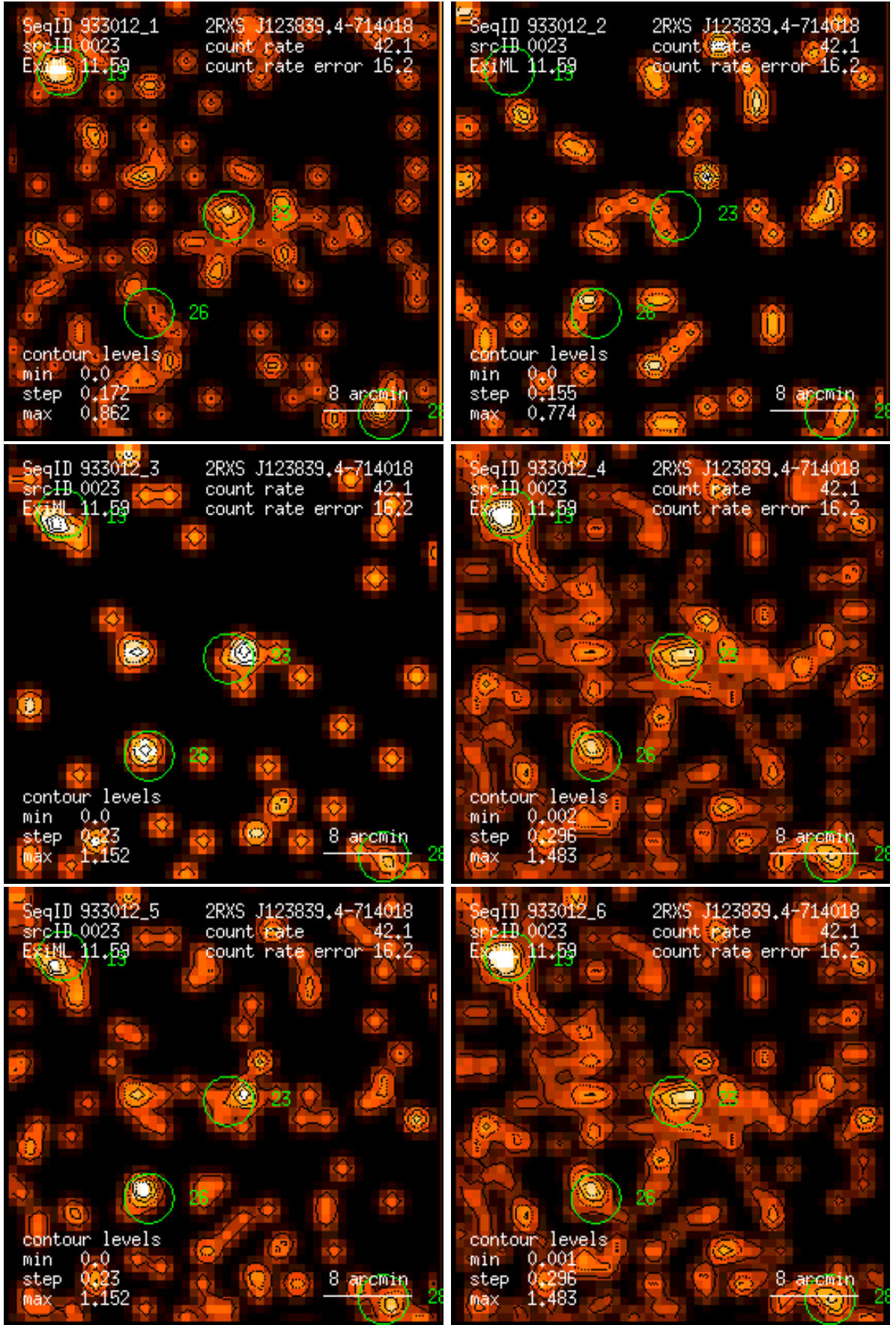
Figure 23: RASS 933012: detection 0023: band rate images, Gaussian filter: (1) PSPC channels 11 – 41, (2) 52 – 90, (3) 91 – 201, (4) 11 – 235, (5) 52 – 201, (6) 11 – 201. Broad band rates in counts/ks. Band rate contour levels in counts/ks/arcmin 2 .
