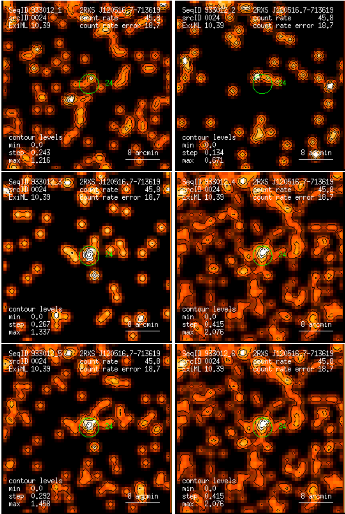
Figure 24: RASS 933012: detection 0024: band rate images, Gaussian filter: (1) PSPC channels 11 – 41, (2) 52 – 90, (3) 91 – 201, (4) 11 – 235, (5) 52 – 201, (6) 11 – 201. Broad band rates in counts/ks. Band rate contour levels in counts/ks/arcmin 2 .
