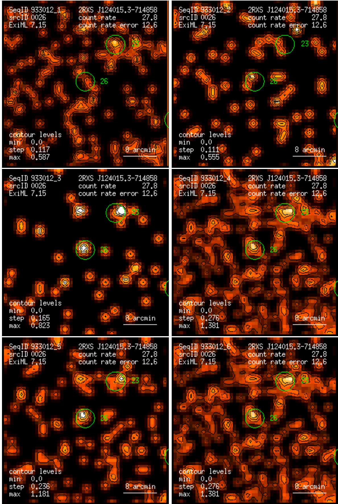
Figure 26: RASS 933012: detection 0026: band rate images, Gaussian filter: (1) PSPC channels 11 – 41, (2) 52 – 90, (3) 91 – 201, (4) 11 – 235, (5) 52 – 201, (6) 11 – 201. Broad band rates in counts/ks. Band rate contour levels in counts/ks/arcmin 2 .
