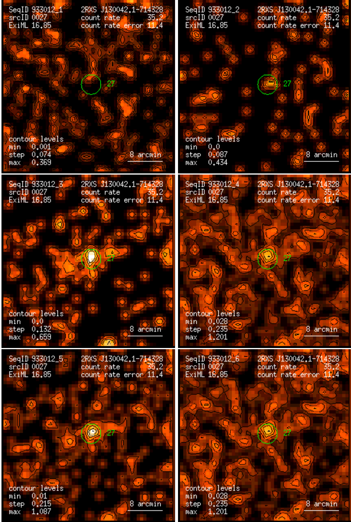
Figure 27: RASS 933012: detection 0027: band rate images, Gaussian filter: (1) PSPC channels 11 – 41, (2) 52 – 90, (3) 91 – 201, (4) 11 – 235, (5) 52 – 201, (6) 11 – 201. Broad band rates in counts/ks. Band rate contour levels in counts/ks/arcmin 2 .
