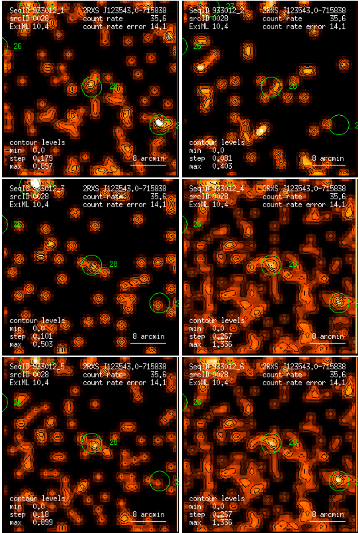
Figure 28: RASS 933012: detection 0028: band rate images, Gaussian filter: (1) PSPC channels 11 – 41, (2) 52 – 90, (3) 91 – 201, (4) 11 – 235, (5) 52 – 201, (6) 11 – 201. Broad band rates in counts/ks. Band rate contour levels in counts/ks/arcmin 2 .
