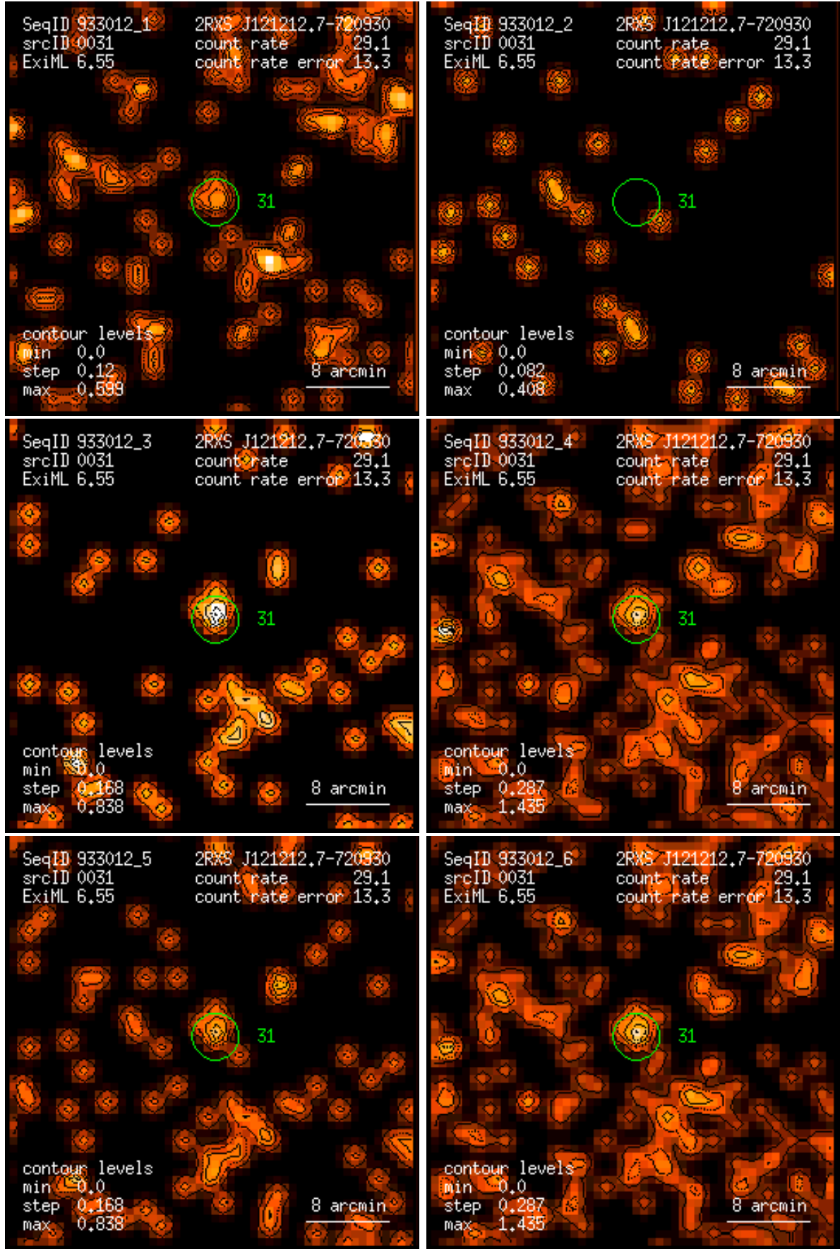
Figure 31: RASS 933012: detection 0031: band rate images, Gaussian filter: (1) PSPC channels 11 – 41, (2) 52 – 90, (3) 91 – 201, (4) 11 – 235, (5) 52 – 201, (6) 11 – 201. Broad band rates in counts/ks. Band rate contour levels in counts/ks/arcmin 2 .
