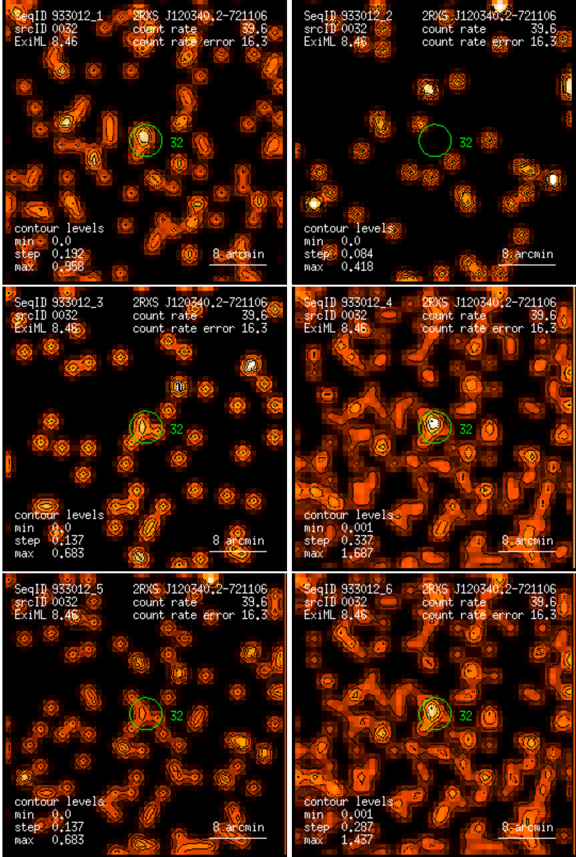
Figure 32: RASS 933012: detection 0032: band rate images, Gaussian filter: (1) PSPC channels 11 – 41, (2) 52 – 90, (3) 91 – 201, (4) 11 – 235, (5) 52 – 201, (6) 11 – 201. Broad band rates in counts/ks. Band rate contour levels in counts/ks/arcmin 2 .
