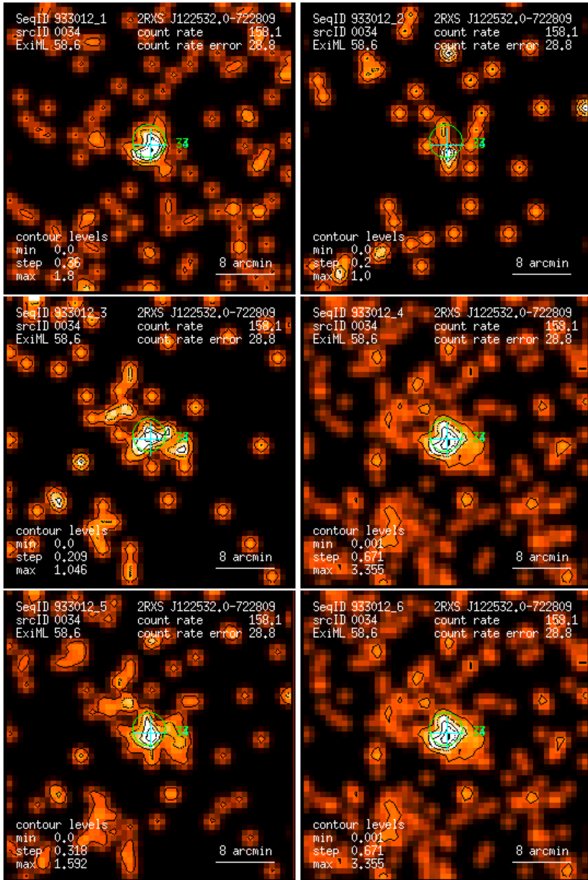
Figure 34: RASS 933012: detection 0034: band rate images, Gaussian filter: (1) PSPC channels 11 – 41, (2) 52 – 90, (3) 91 – 201, (4) 11 – 235, (5) 52 – 201, (6) 11 – 201. Broad band rates in counts/ks. Band rate contour levels in counts/ks/arcmin 2 .
