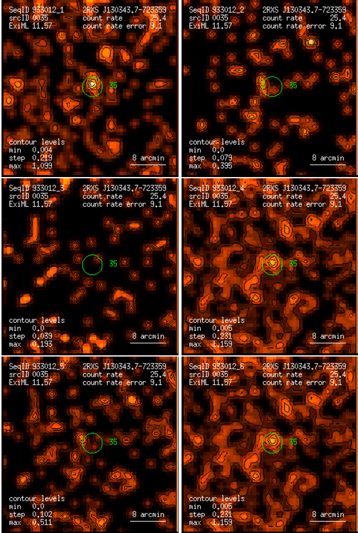
Figure 35: RASS 933012: detection 0035: band rate images, Gaussian filter: (1) PSPC channels 11 – 41, (2) 52 – 90, (3) 91 – 201, (4) 11 – 235, (5) 52 – 201, (6) 11 – 201. Broad band rates in counts/ks. Band rate contour levels in counts/ks/arcmin 2 .
