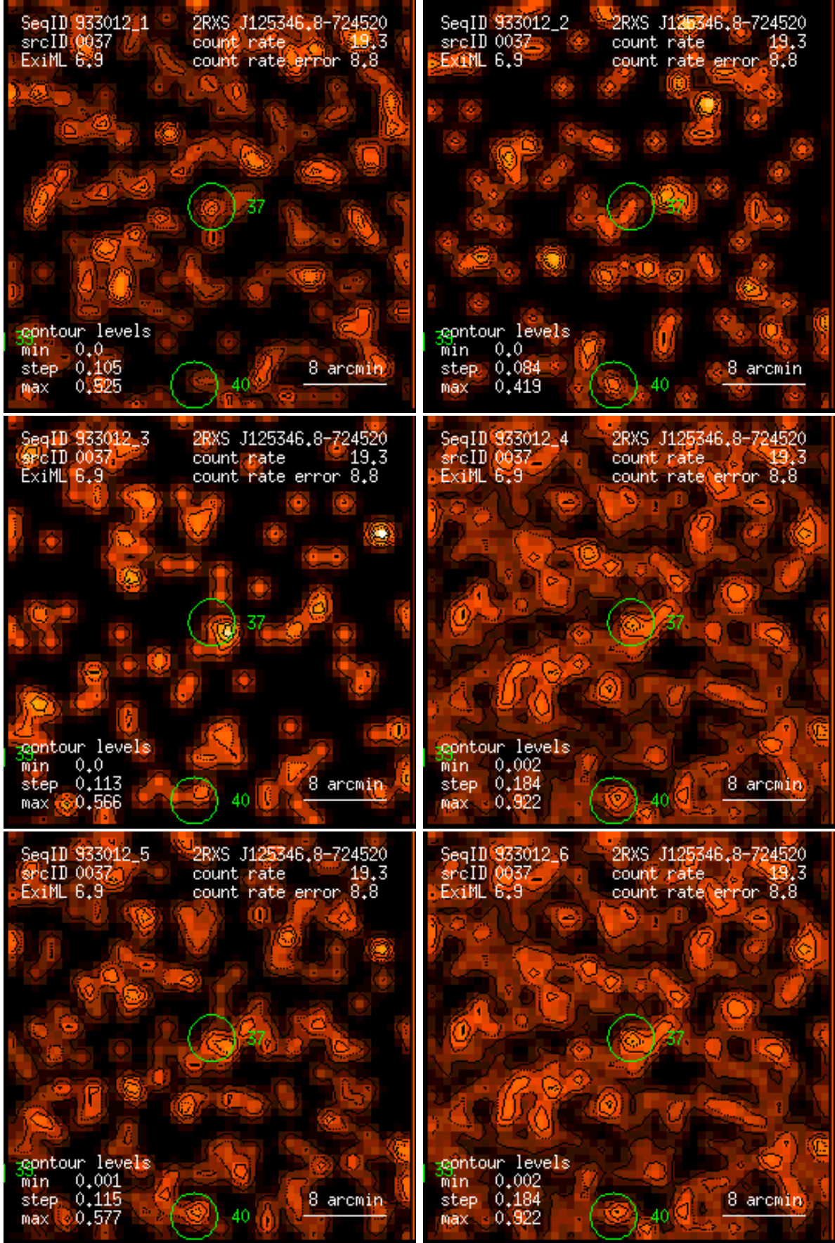
Figure 37: RASS 933012: detection 0037: band rate images, Gaussian filter: (1) PSPC channels 11 – 41, (2) 52 – 90, (3) 91 – 201, (4) 11 – 235, (5) 52 – 201, (6) 11 – 201. Broad band rates in counts/ks. Band rate contour levels in counts/ks/arcmin 2 .
