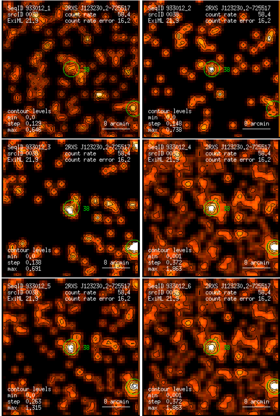
Figure 38: RASS 933012: detection 0038: band rate images, Gaussian filter: (1) PSPC channels 11 – 41, (2) 52 – 90, (3) 91 – 201, (4) 11 – 235, (5) 52 – 201, (6) 11 – 201. Broad band rates in counts/ks. Band rate contour levels in counts/ks/arcmin 2 .
