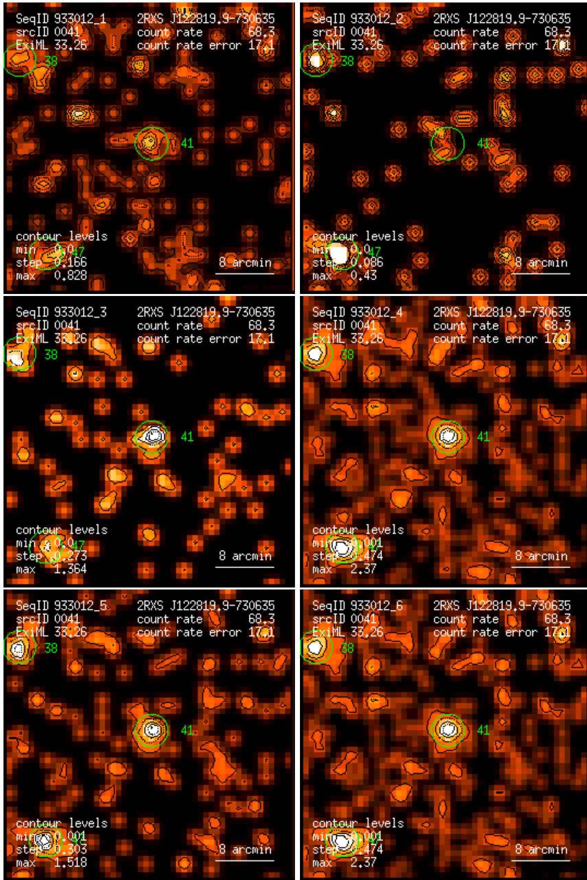
Figure 41: RASS 933012: detection 0041: band rate images, Gaussian filter: (1) PSPC channels 11 – 41, (2) 52 – 90, (3) 91 – 201, (4) 11 – 235, (5) 52 – 201, (6) 11 – 201. Broad band rates in counts/ks. Band rate contour levels in counts/ks/arcmin 2 .
