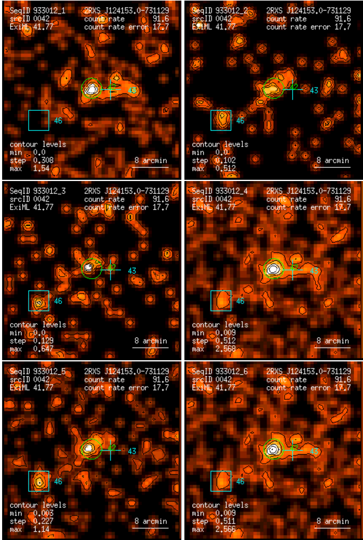
Figure 42: RASS 933012: detection 0042: band rate images, Gaussian filter: (1) PSPC channels 11 – 41, (2) 52 – 90, (3) 91 – 201, (4) 11 – 235, (5) 52 – 201, (6) 11 – 201. Broad band rates in counts/ks. Band rate contour levels in counts/ks/arcmin 2 .
