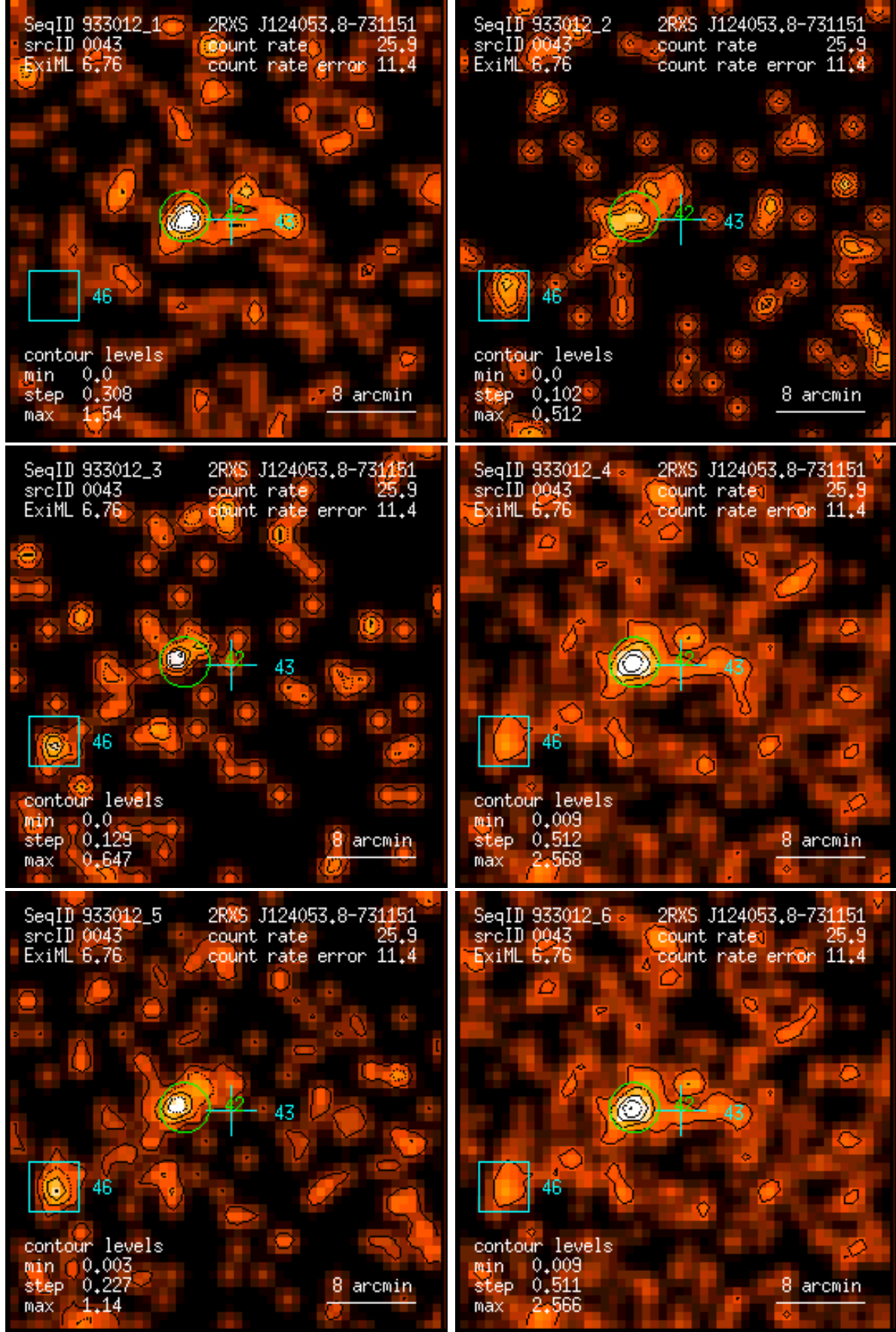
Figure 43: RASS 933012: detection 0043: band rate images, Gaussian filter: (1) PSPC channels 11 – 41, (2) 52 – 90, (3) 91 – 201, (4) 11 – 235, (5) 52 – 201, (6) 11 – 201. Broad band rates in counts/ks. Band rate contour levels in counts/ks/arcmin 2 .
