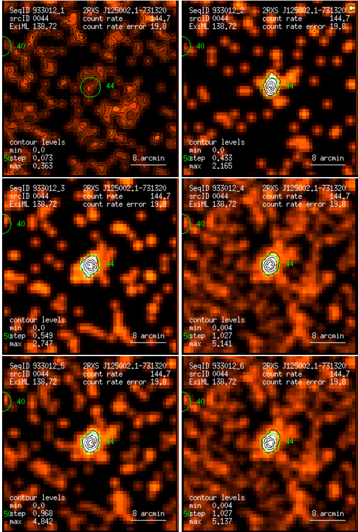
Figure 44: RASS 933012: detection 0044: band rate images, Gaussian filter: (1) PSPC channels 11 – 41, (2) 52 – 90, (3) 91 – 201, (4) 11 – 235, (5) 52 – 201, (6) 11 – 201. Broad band rates in counts/ks. Band rate contour levels in counts/ks/arcmin 2 .
