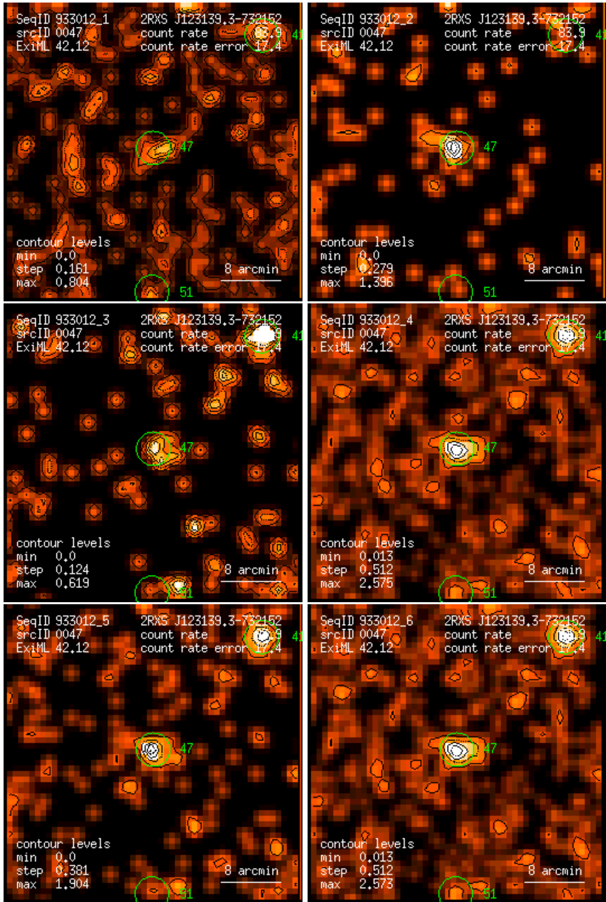
Figure 47: RASS 933012: detection 0047: band rate images, Gaussian filter: (1) PSPC channels 11 – 41, (2) 52 – 90, (3) 91 – 201, (4) 11 – 235, (5) 52 – 201, (6) 11 – 201. Broad band rates in counts/ks. Band rate contour levels in counts/ks/arcmin 2 .
