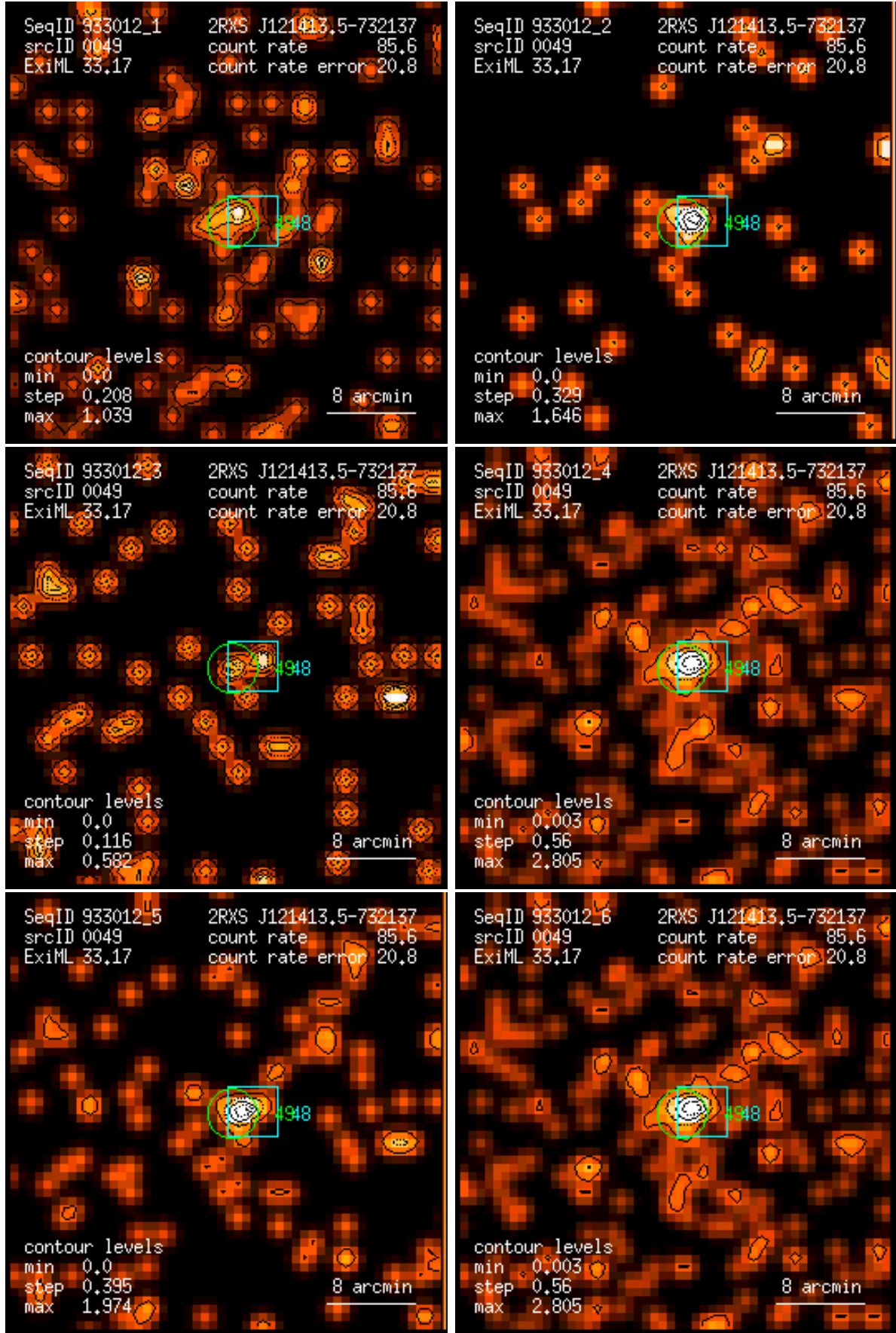
Figure 49: RASS 933012: detection 0049: band rate images, Gaussian filter: (1) PSPC channels 11 – 41, (2) 52 – 90, (3) 91 – 201, (4) 11 – 235, (5) 52 – 201, (6) 11 – 201. Broad band rates in counts/ks. Band rate contour levels in counts/ks/arcmin 2 .
