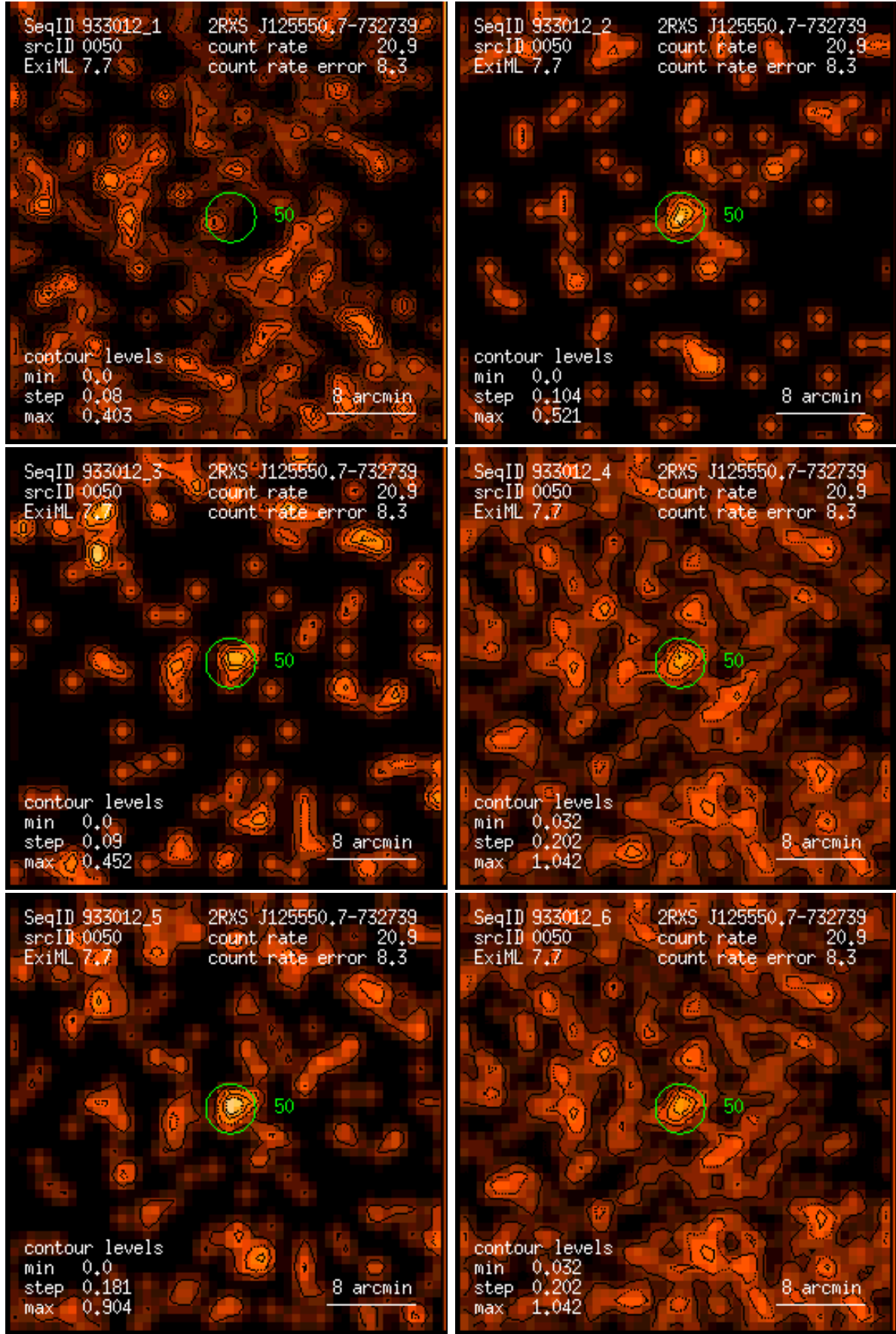
Figure 50: RASS 933012: detection 0050: band rate images, Gaussian filter: (1) PSPC channels 11 – 41, (2) 52 – 90, (3) 91 – 201, (4) 11 – 235, (5) 52 – 201, (6) 11 – 201. Broad band rates in counts/ks. Band rate contour levels in counts/ks/arcmin 2 .
