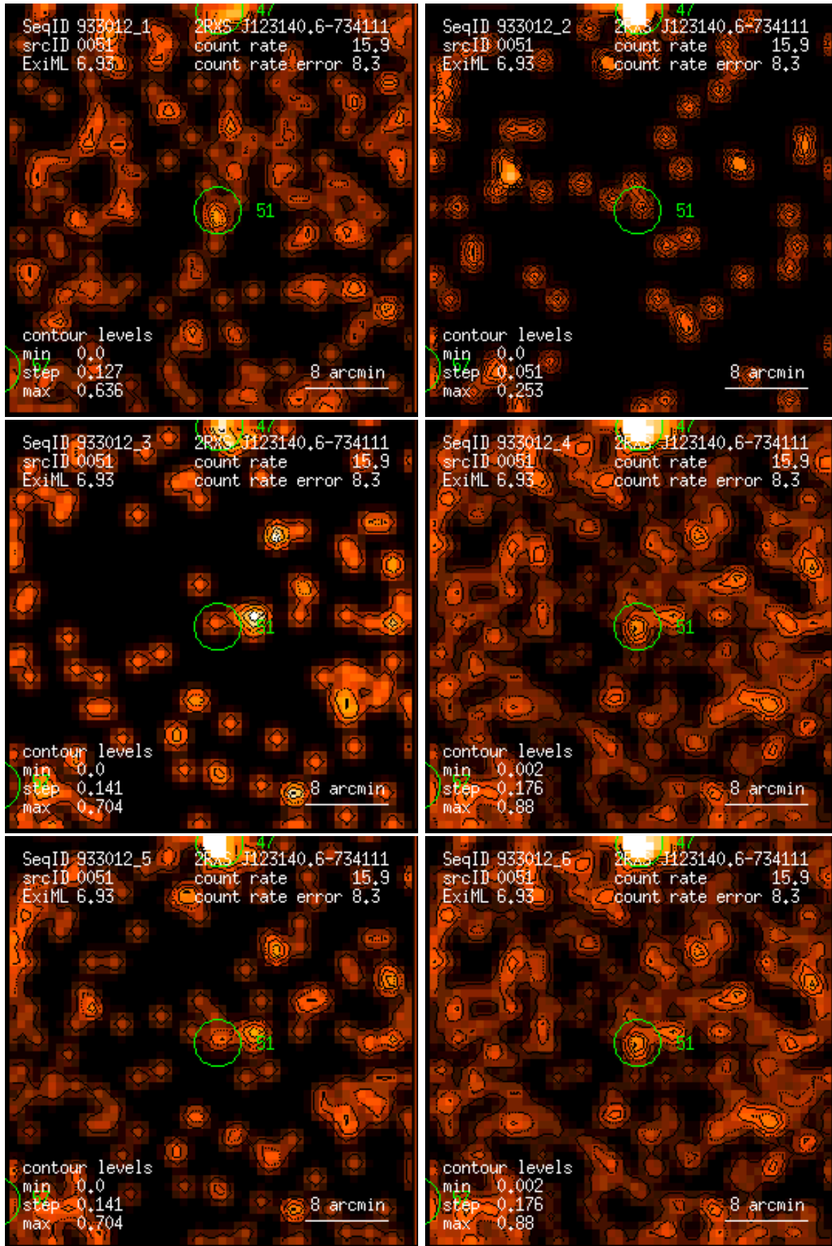
Figure 51: RASS 933012: detection 0051: band rate images, Gaussian filter: (1) PSPC channels 11 – 41, (2) 52 – 90, (3) 91 – 201, (4) 11 – 235, (5) 52 – 201, (6) 11 – 201. Broad band rates in counts/ks. Band rate contour levels in counts/ks/arcmin 2 .
