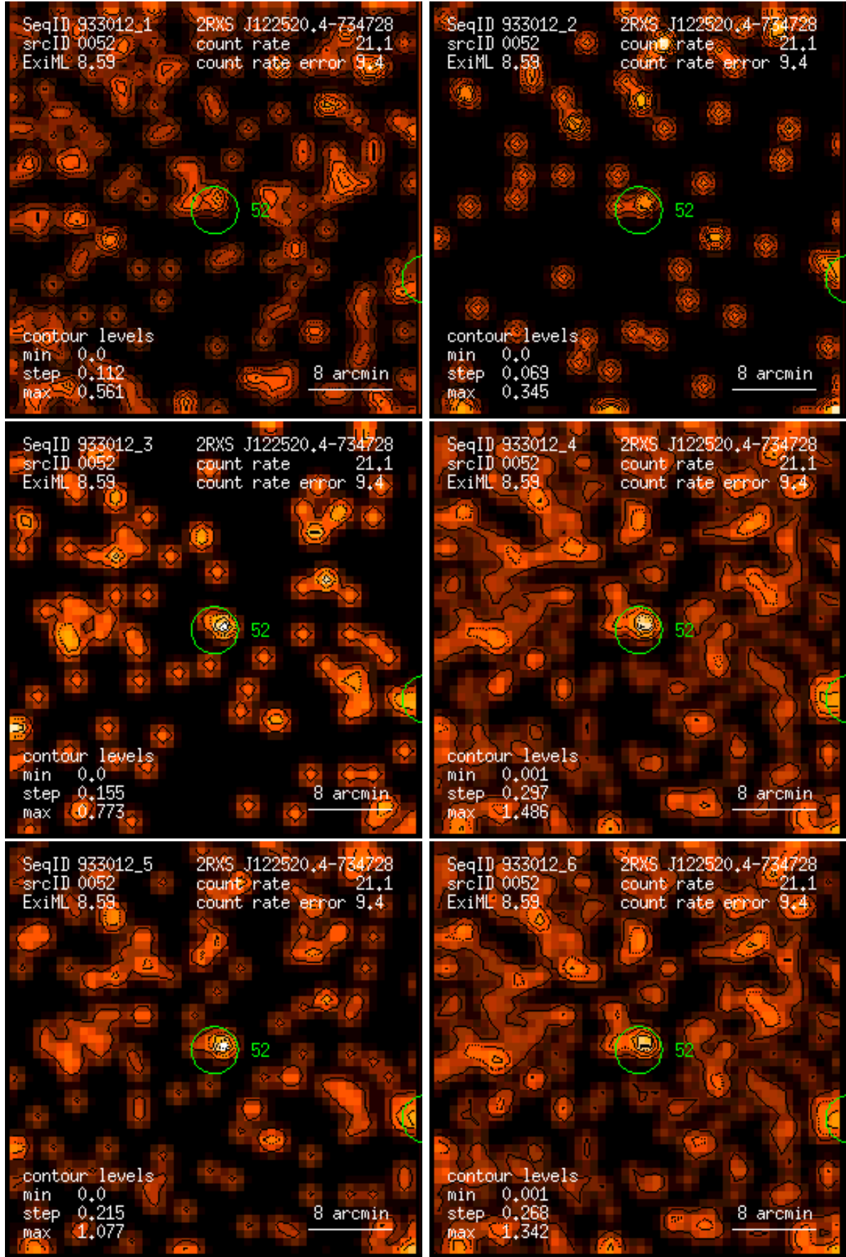
Figure 52: RASS 933012: detection 0052: band rate images, Gaussian filter: (1) PSPC channels 11 – 41, (2) 52 – 90, (3) 91 – 201, (4) 11 – 235, (5) 52 – 201, (6) 11 – 201. Broad band rates in counts/ks. Band rate contour levels in counts/ks/arcmin 2 .
