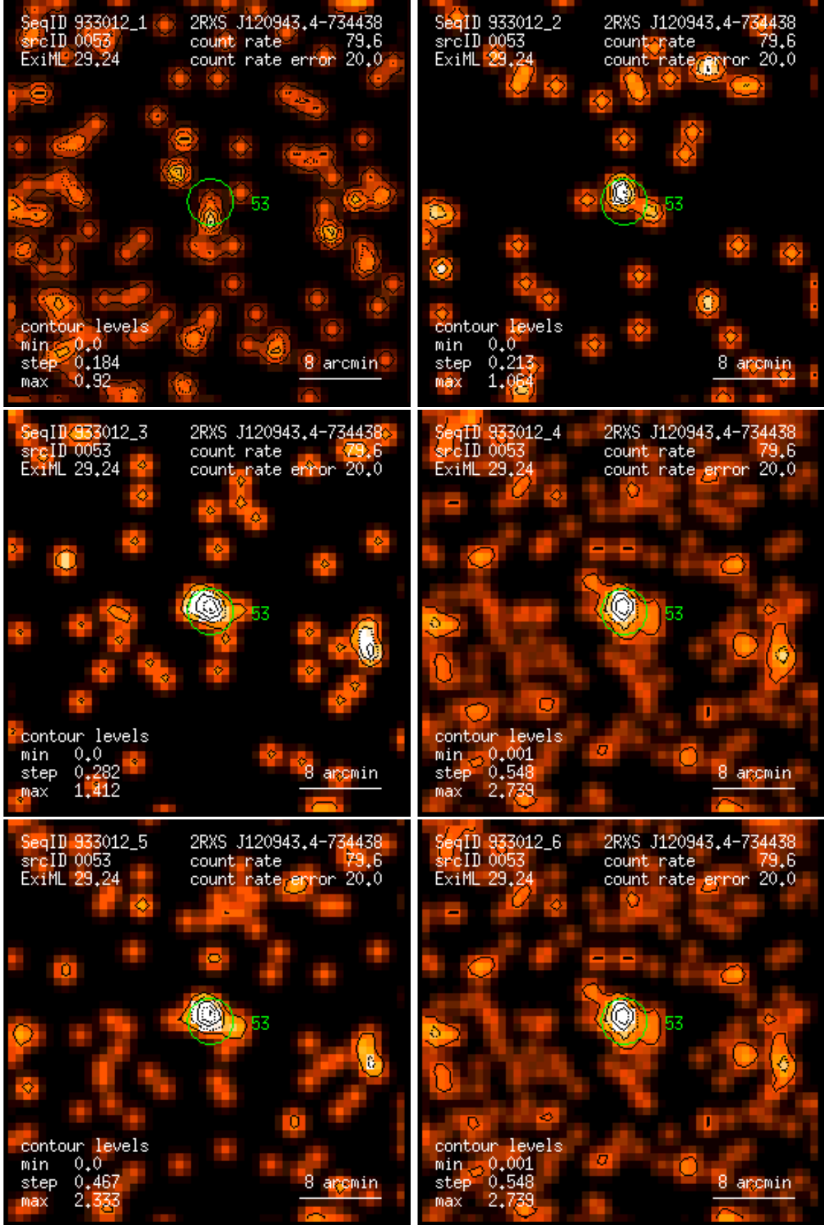
Figure 53: RASS 933012: detection 0053: band rate images, Gaussian filter: (1) PSPC channels 11 – 41, (2) 52 – 90, (3) 91 – 201, (4) 11 – 235, (5) 52 – 201, (6) 11 – 201. Broad band rates in counts/ks. Band rate contour levels in counts/ks/arcmin 2 .
