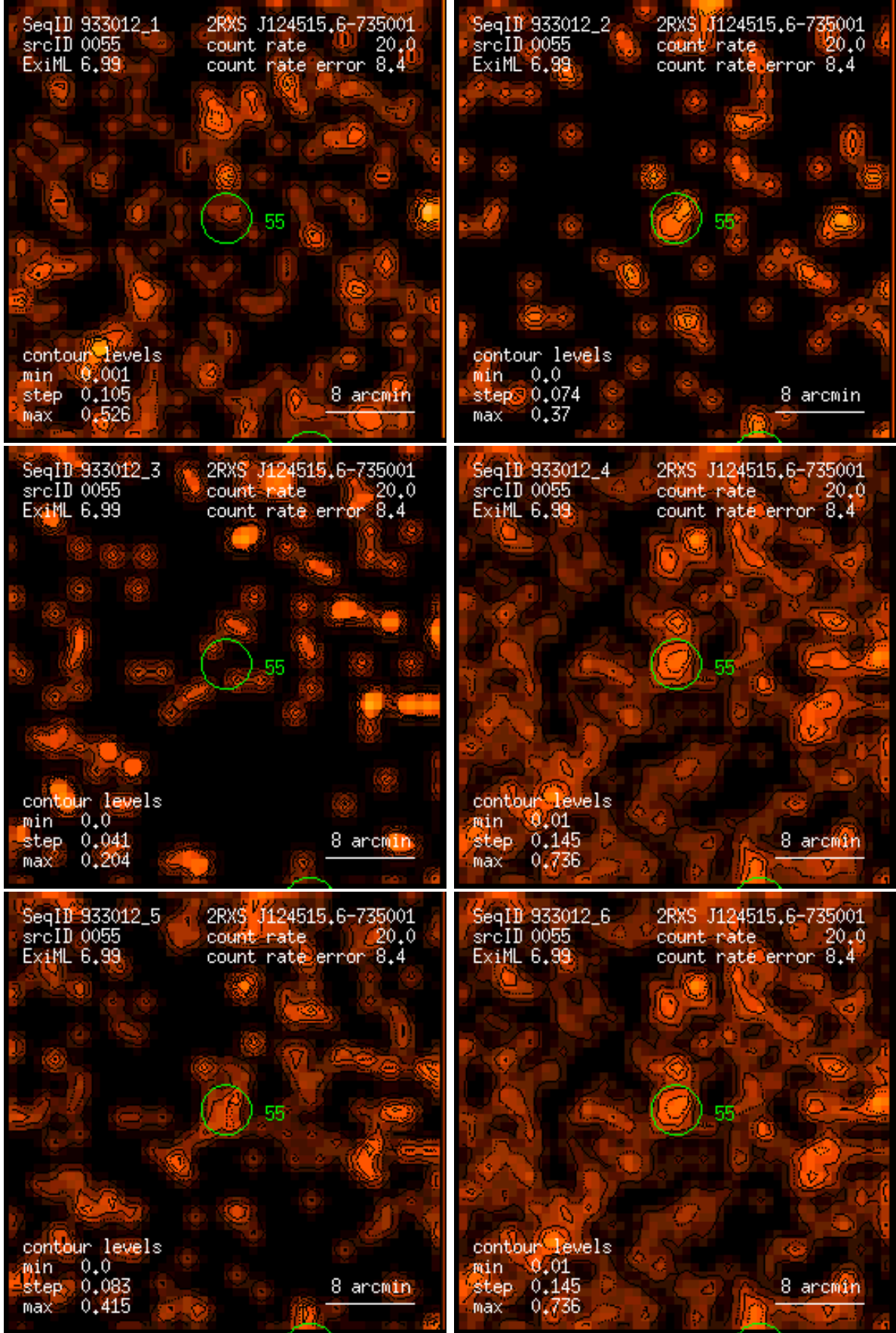
Figure 55: RASS 933012: detection 0055: band rate images, Gaussian filter: (1) PSPC channels 11 – 41, (2) 52 – 90, (3) 91 – 201, (4) 11 – 235, (5) 52 – 201, (6) 11 – 201. Broad band rates in counts/ks. Band rate contour levels in counts/ks/arcmin 2 .
