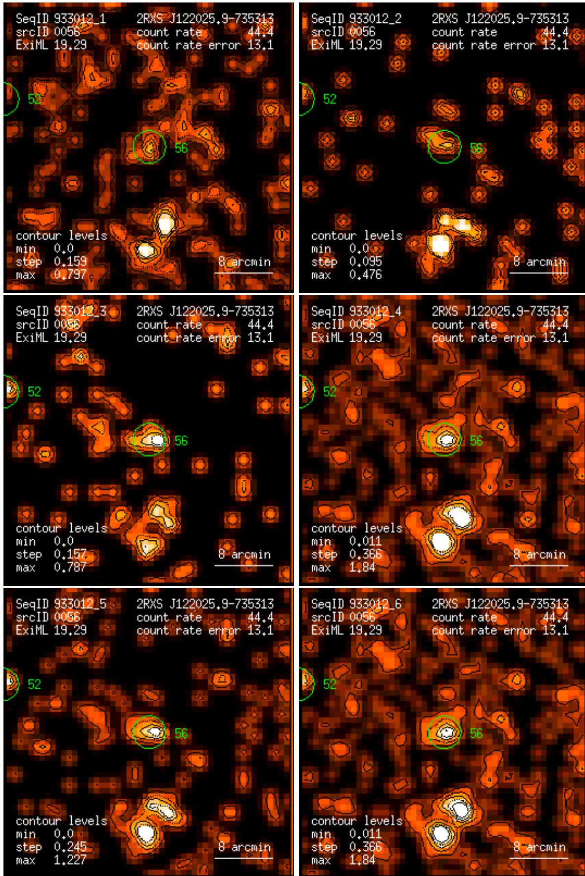
Figure 56: RASS 933012: detection 0056: band rate images, Gaussian filter: (1) PSPC channels 11 – 41, (2) 52 – 90, (3) 91 – 201, (4) 11 – 235, (5) 52 – 201, (6) 11 – 201. Broad band rates in counts/ks. Band rate contour levels in counts/ks/arcmin 2 .
