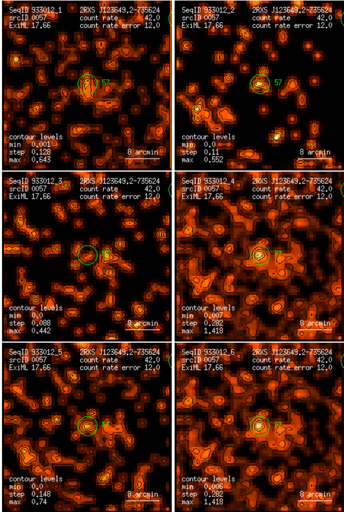
Figure 57: RASS 933012: detection 0057: band rate images, Gaussian filter: (1) PSPC channels 11 – 41, (2) 52 – 90, (3) 91 – 201, (4) 11 – 235, (5) 52 – 201, (6) 11 – 201. Broad band rates in counts/ks. Band rate contour levels in counts/ks/arcmin 2 .
