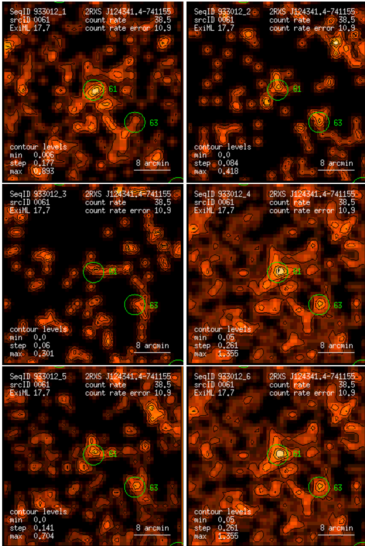
Figure 61: RASS 933012: detection 0061: band rate images, Gaussian filter: (1) PSPC channels 11 – 41, (2) 52 – 90, (3) 91 – 201, (4) 11 – 235, (5) 52 – 201, (6) 11 – 201. Broad band rates in counts/ks. Band rate contour levels in counts/ks/arcmin 2 .
