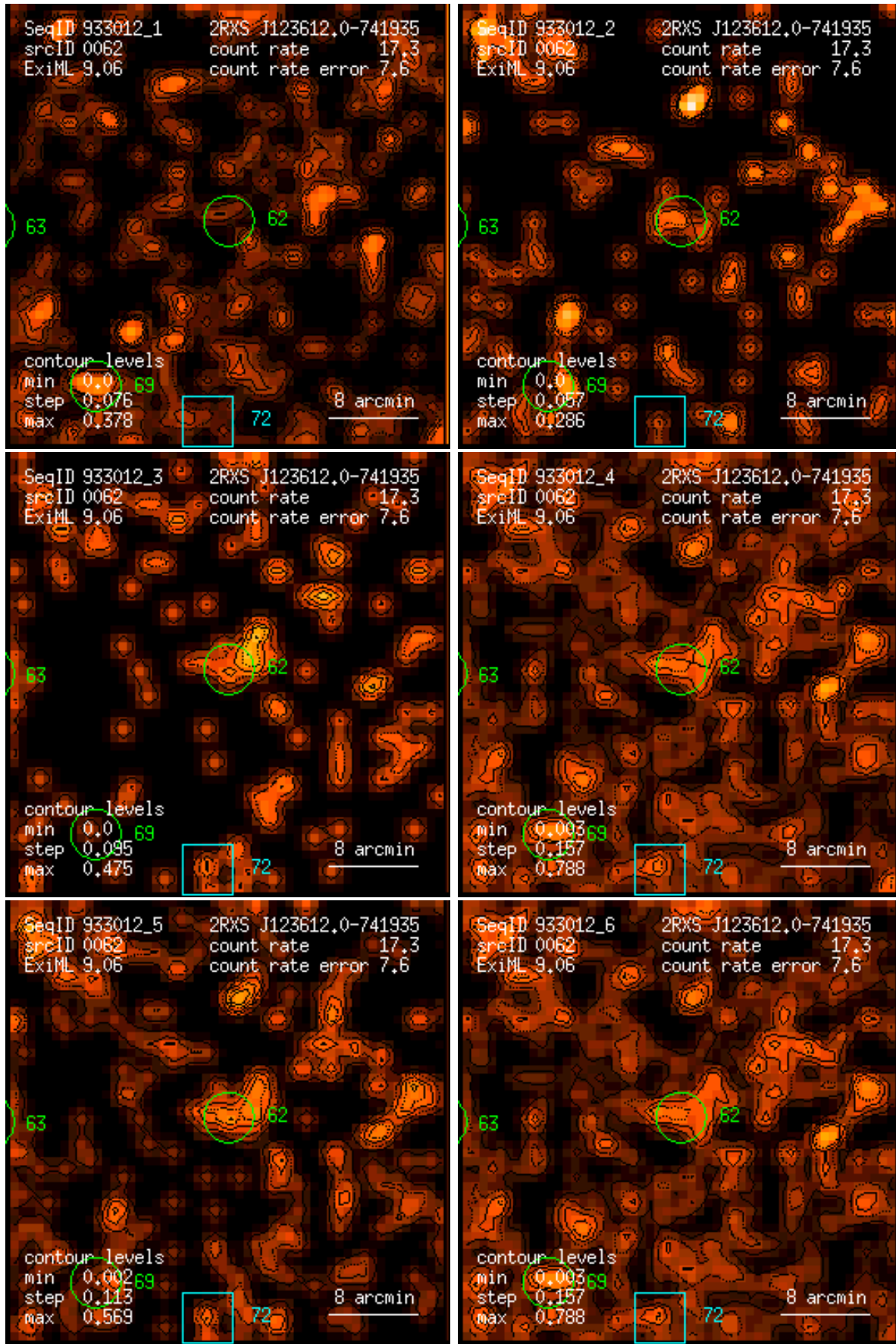
Figure 62: RASS 933012: detection 0062: band rate images, Gaussian filter: (1) PSPC channels 11 – 41, (2) 52 – 90, (3) 91 – 201, (4) 11 – 235, (5) 52 – 201, (6) 11 – 201. Broad band rates in counts/ks. Band rate contour levels in counts/ks/arcmin 2 .
