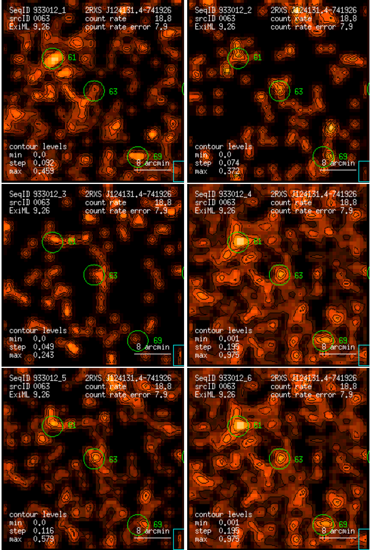
Figure 63: RASS 933012: detection 0063: band rate images, Gaussian filter: (1) PSPC channels 11 – 41, (2) 52 – 90, (3) 91 – 201, (4) 11 – 235, (5) 52 – 201, (6) 11 – 201. Broad band rates in counts/ks. Band rate contour levels in counts/ks/arcmin 2 .
