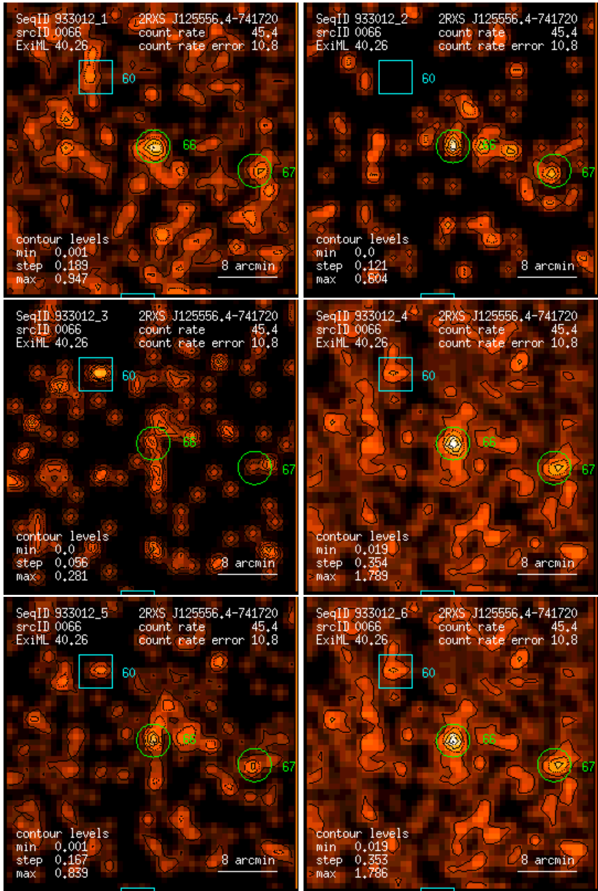
Figure 66: RASS 933012: detection 0066: band rate images, Gaussian filter: (1) PSPC channels 11 – 41, (2) 52 – 90, (3) 91 – 201, (4) 11 – 235, (5) 52 – 201, (6) 11 – 201. Broad band rates in counts/ks. Band rate contour levels in counts/ks/arcmin 2 .
