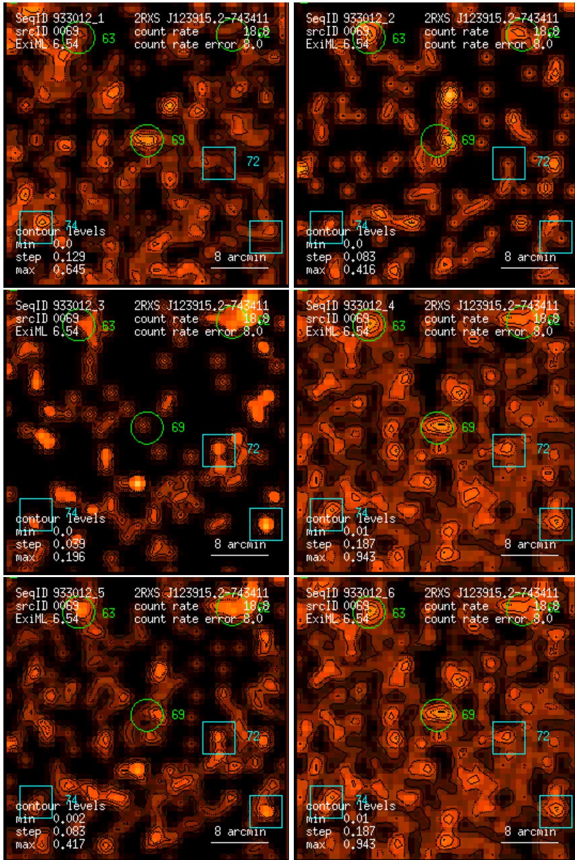
Figure 69: RASS 933012: detection 0069: band rate images, Gaussian filter: (1) PSPC channels 11 – 41, (2) 52 – 90, (3) 91 – 201, (4) 11 – 235, (5) 52 – 201, (6) 11 – 201. Broad band rates in counts/ks. Band rate contour levels in counts/ks/arcmin 2 .
