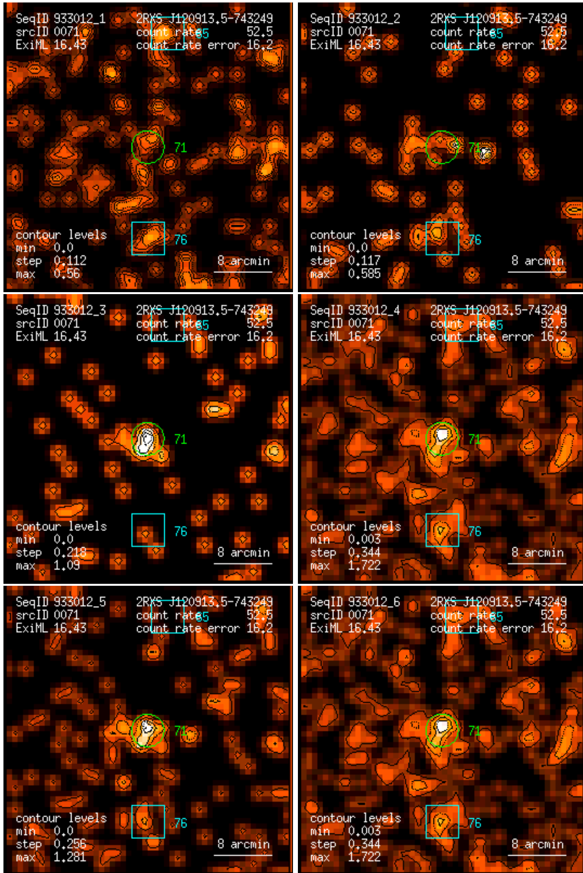
Figure 71: RASS 933012: detection 0071: band rate images, Gaussian filter: (1) PSPC channels 11 – 41, (2) 52 – 90, (3) 91 – 201, (4) 11 – 235, (5) 52 – 201, (6) 11 – 201. Broad band rates in counts/ks. Band rate contour levels in counts/ks/arcmin 2 .
