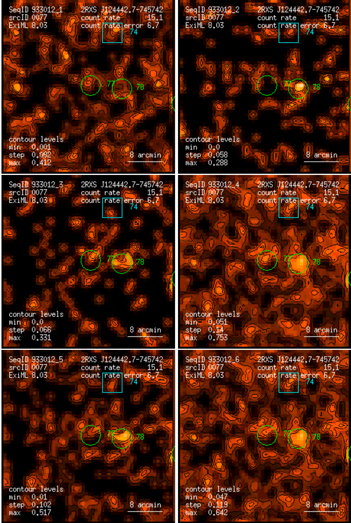
Figure 77: RASS 933012: detection 0077: band rate images, Gaussian filter: (1) PSPC channels 11 – 41, (2) 52 – 90, (3) 91 – 201, (4) 11 – 235, (5) 52 – 201, (6) 11 – 201. Broad band rates in counts/ks. Band rate contour levels in counts/ks/arcmin 2 .
