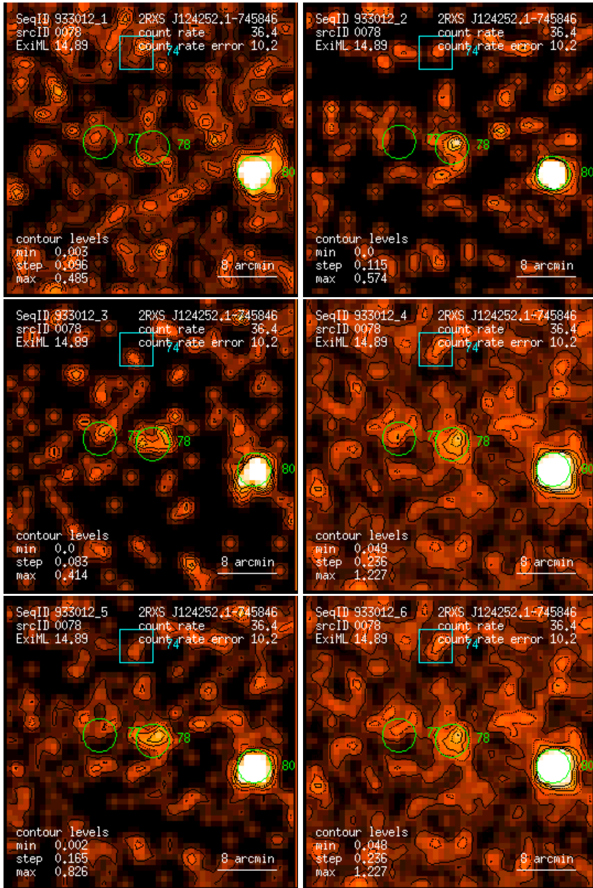
Figure 78: RASS 933012: detection 0078: band rate images, Gaussian filter: (1) PSPC channels 11 – 41, (2) 52 – 90, (3) 91 – 201, (4) 11 – 235, (5) 52 – 201, (6) 11 – 201. Broad band rates in counts/ks. Band rate contour levels in counts/ks/arcmin 2 .
