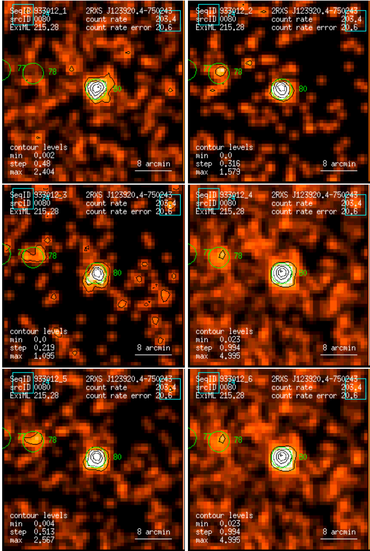
Figure 80: RASS 933012: detection 0080: band rate images, Gaussian filter: (1) PSPC channels 11 – 41, (2) 52 – 90, (3) 91 – 201, (4) 11 – 235, (5) 52 – 201, (6) 11 – 201. Broad band rates in counts/ks. Band rate contour levels in counts/ks/arcmin 2 .
