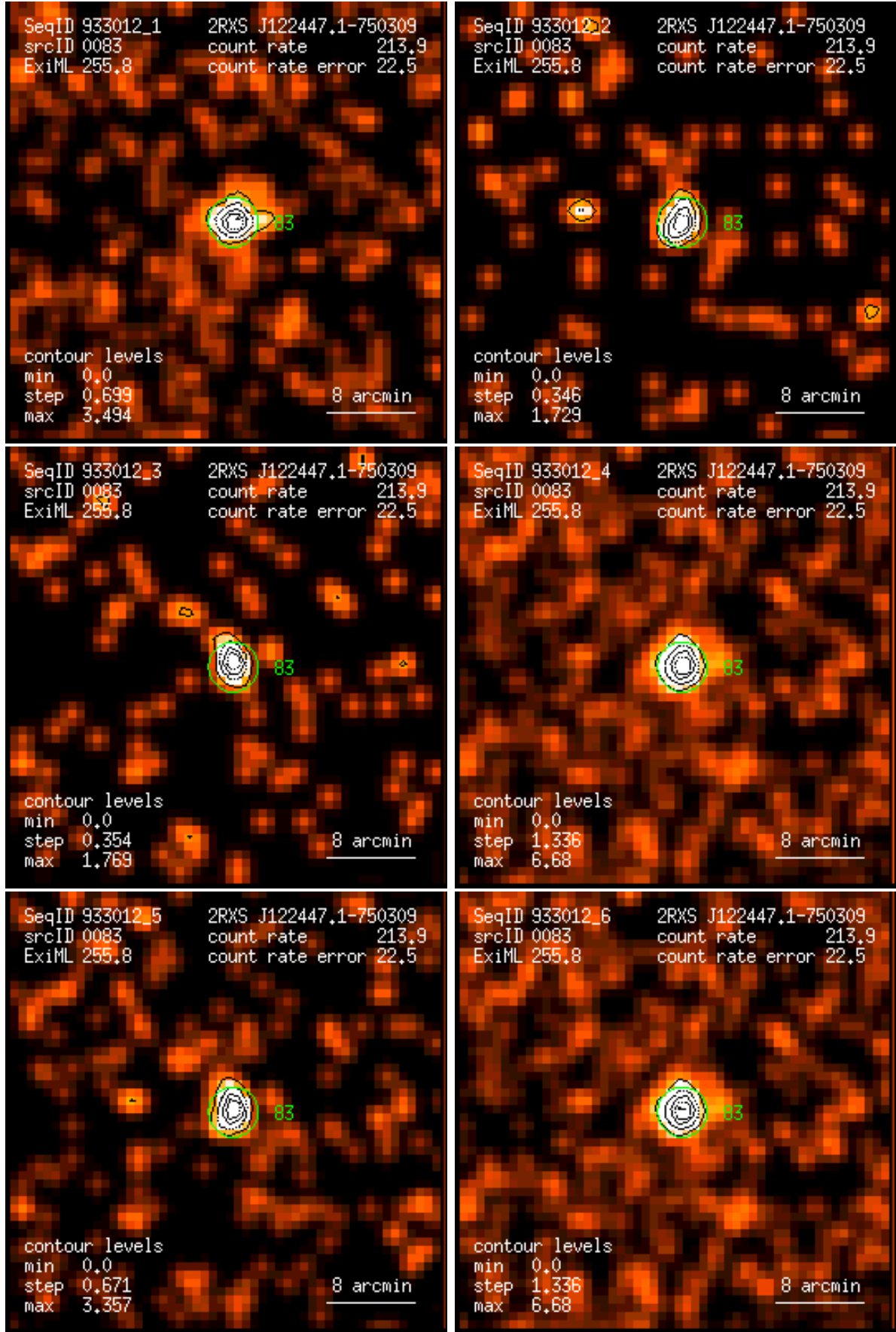
Figure 83: RASS 933012: detection 0083: band rate images, Gaussian filter: (1) PSPC channels 11 – 41, (2) 52 – 90, (3) 91 – 201, (4) 11 – 235, (5) 52 – 201, (6) 11 – 201. Broad band rates in counts/ks. Band rate contour levels in counts/ks/arcmin 2 .
